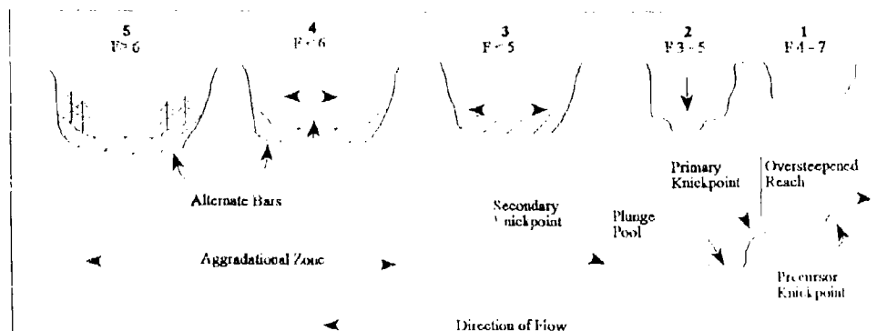
Figure 3.1c Schematic Longitudinal Profile of an Active Channel Showing Identifiable Features (modified from Schumm, 1984)
