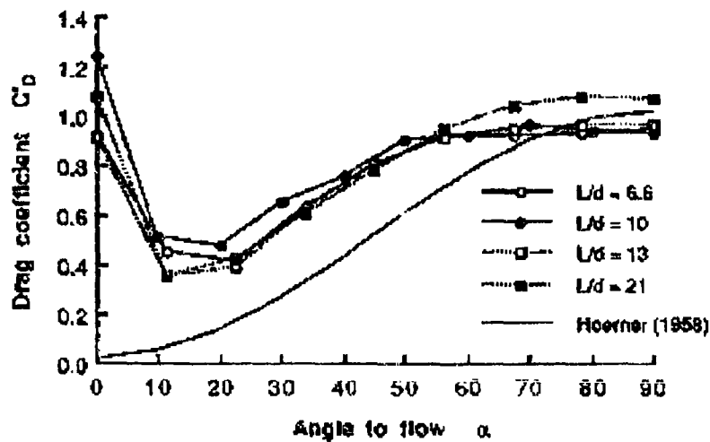
Figure 2 : Variation in drag coefficient with angle of rotation for cylinders of various lengths and diameters. Hoerner's (1958) relationship is for infinitely long cylinders.
