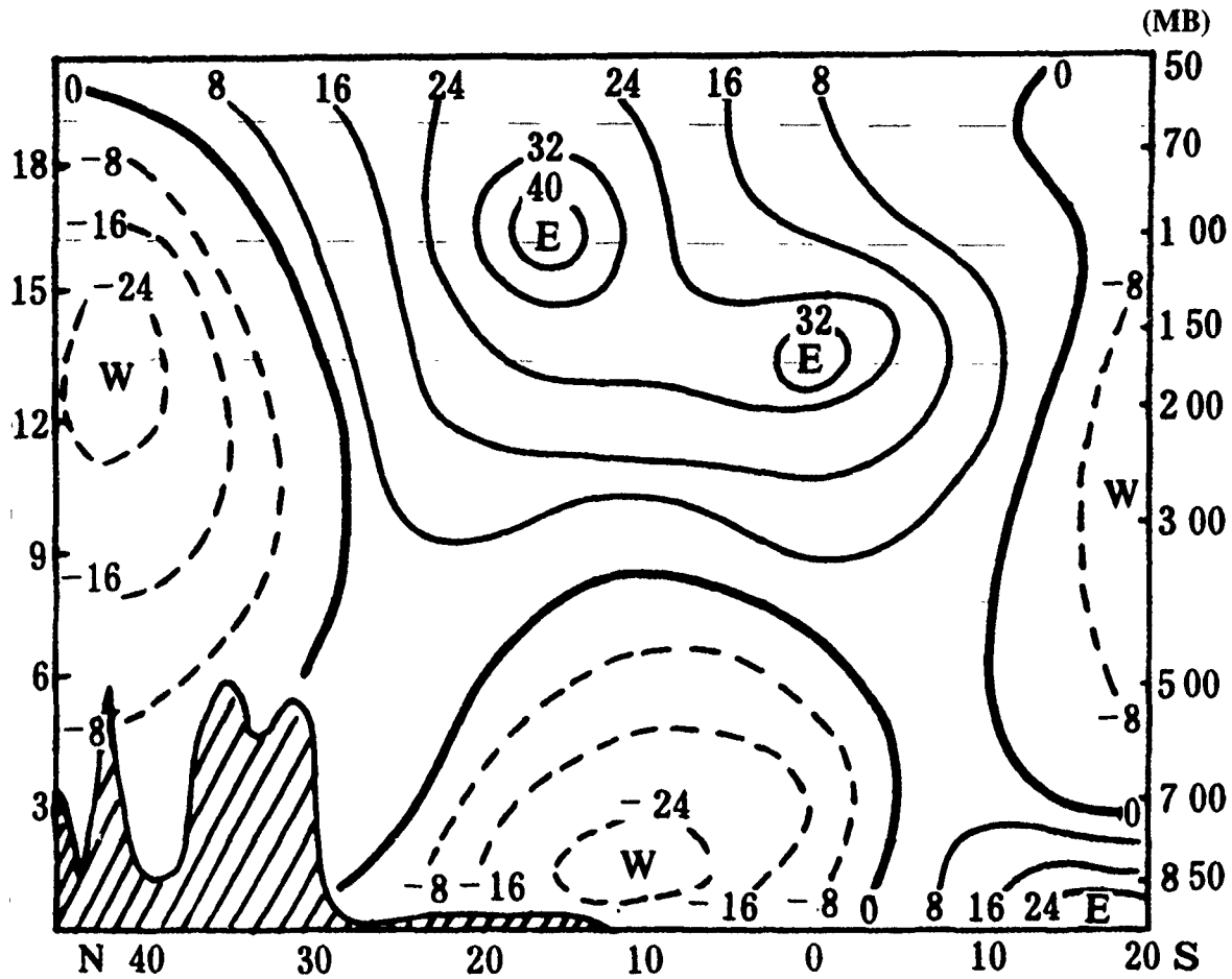
Figure 2-11. A Cross Section of the Mean Zonal Wind Components along 80° E for July. Solid (dashed) lines denotes isotach of easterly wind (westerly wind). Units: m s -1 .
