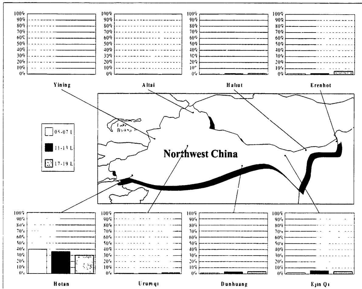
Figure 4-15. April Visibility below 4,800 Meters. The graphs show a breakdown of visibility below 4,800 meters based on location and diurnal influences.
