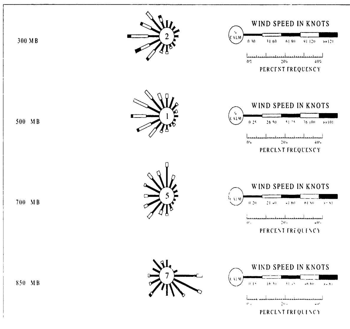
Figure 5-25. July Upper-Air Wind Roses. The upper-air wind roses depict wind speeds and directions for standard pressure surfaces between 850 and 300 mb at Ulan-Bator. Each wind rose has a tailored legend.
