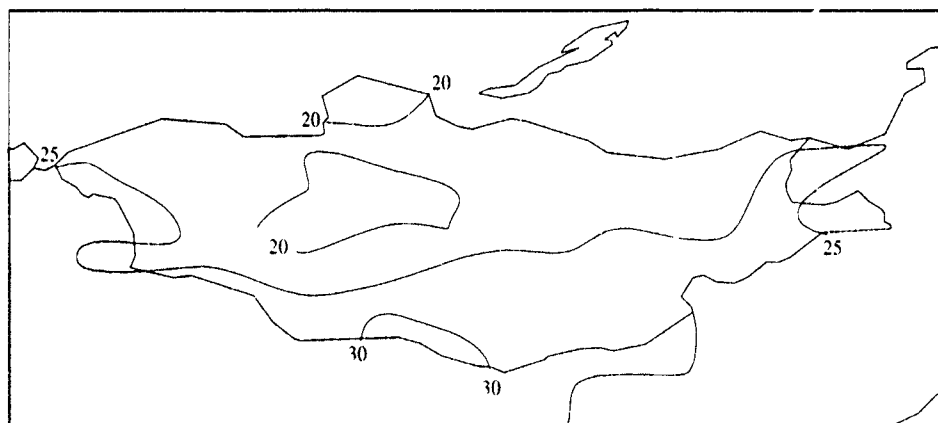
Figure 5-28. July Mean Maximum Temperatures in (°C). The isopleths show the average of all high temperatures for the most representative month of the season.
