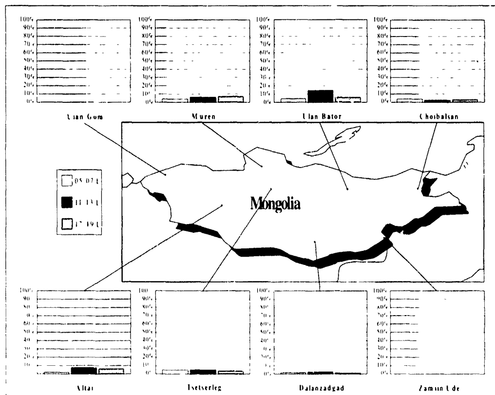
Figure 5-22. July Visibility below 4,800 Meters. The graphs show a breakdown of visibility below 4,800 meters based on location and diurnal influences.
