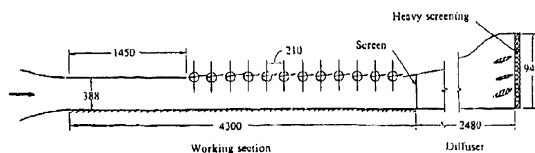
Figure 1: Details of working section (dimensions in mm).
