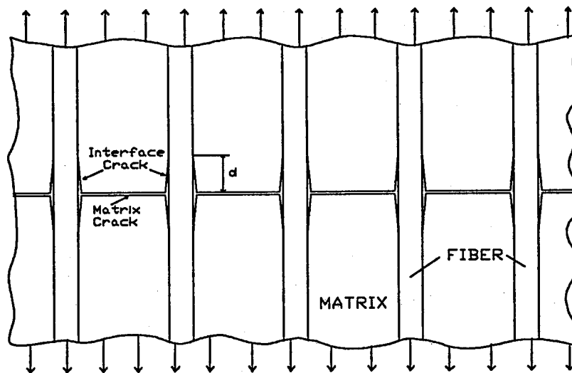
Fig. 3.2 H-shaped cracks
