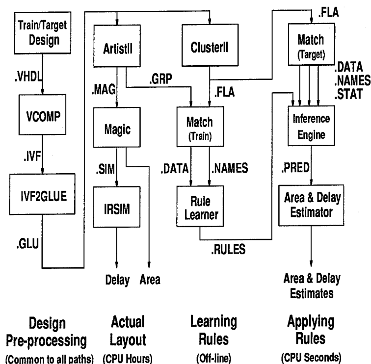
Figure 44 Solution Architecture
