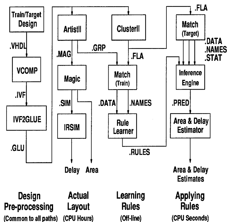
Figure 15 Solution Architecture
