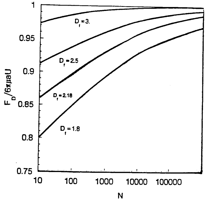
Fig. 2 Drag reduction associated with effective permeability for a quasi-spherical "fractal" aggregate comprised of N primary spheres in the continuum regime ( a = R_{max} = \{(3/2) \cdot [D_f + 2] / D_f\}^{1/2} R_{gyration} ) (after Tandon and Rosner, 1994)
