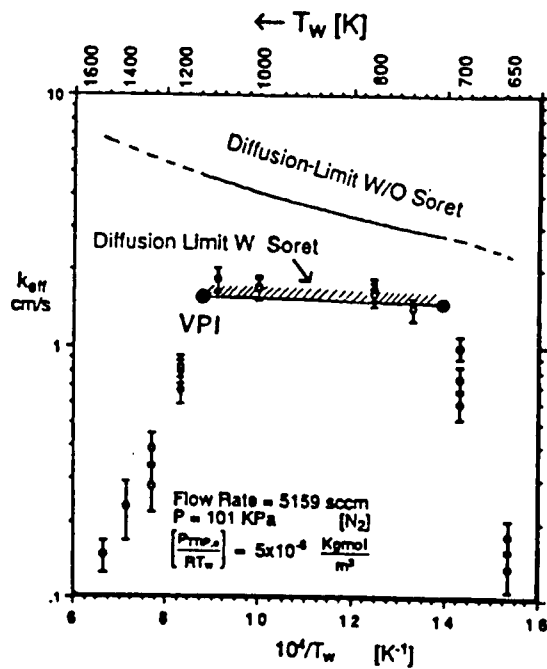
Fig. 3: TiO 2 Deposition rate data from TTIP/O 2 /N 2 with calculated diffusion-controlled limits showing effect of Soret diffusion
