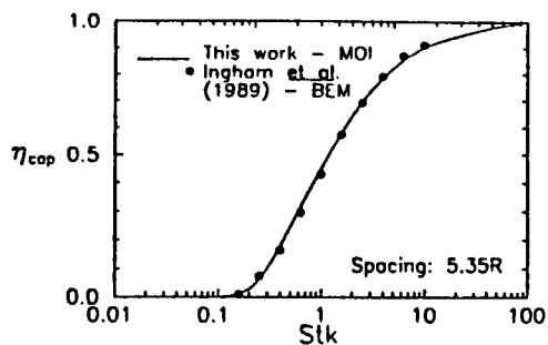
Fig. 5. Comparison of present capture efficiency calculation to the results of Ingham et al. (1989) for S \approx 5.35 .
