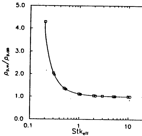
Fig. 10. Correlation of stagnation point particle concentration enrichment \rho_{p,w}/\rho_{p,\infty} for the central cylinder, in an array of three collectors, at S=2.5 (squares), 4 (circles), \alpha (triangles), in terms of Stk_{eff} .
