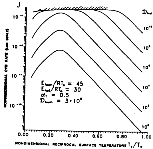
Fig. 1: CSL-theory predicted Arrhenius behavior for CVD-rates in the presence (at high surface temperatures) of vapor phase reactions yielding non-depositing products (2); Dependence of nondimensional CVD-rate (log scale) on (reciprocal) surface temperature and heterogeneous reaction Damkohler number A_{het}\delta/D , where A_{het} is the pre-exponential factor of the first-order heterogeneous rate constant.
