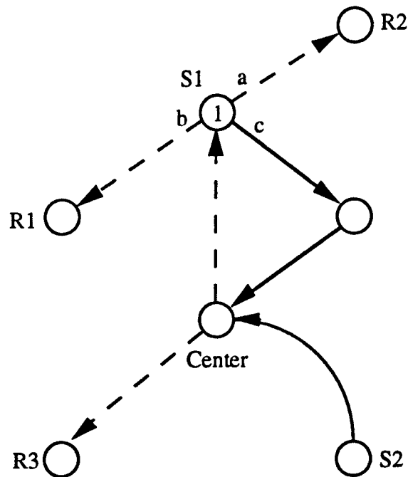
Figure 1. Tree Construction
