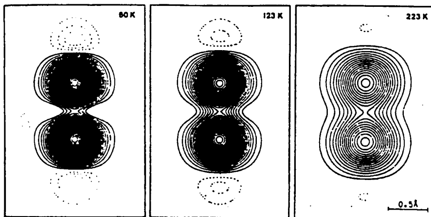
Figure 18. Probability density map of H1 in the (10\bar{1}0) plane as described by harmonic and anharmonic terms up to fourth order (equidistant contours, zero contour omitted). The small negative regions are due to minor shortcomings of the chosen mathematical description. With the limits of error, these probability densities are following the expectations for simple temperature dependence assuming Boltzmann statistics (after Kuhs and Lehmann 1983).
