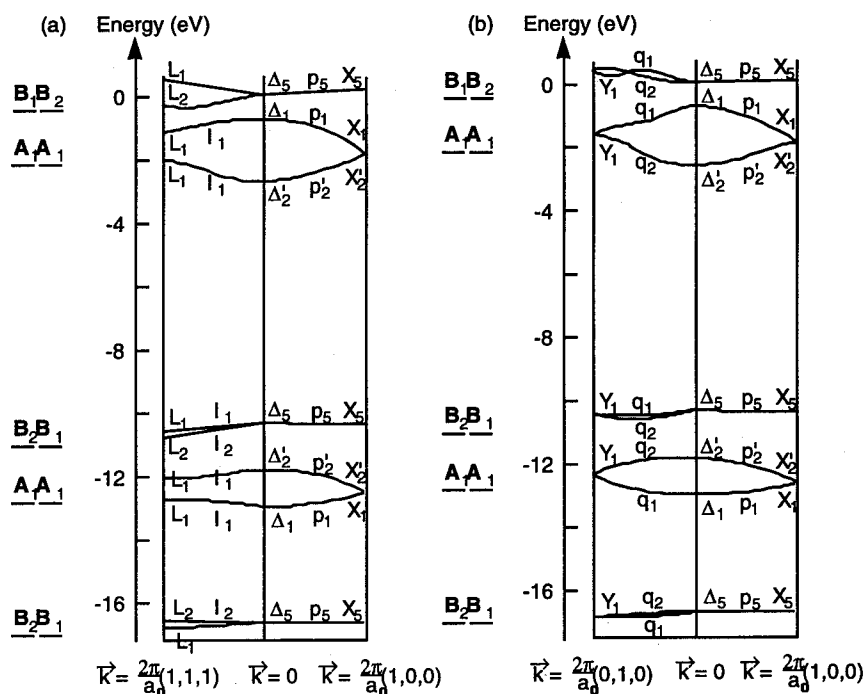
Figure 25. Valance and excited bands of the cubic-ice model structure at the points shown in Figure 26 (after Pastori Parravicini and Resca 1973).
