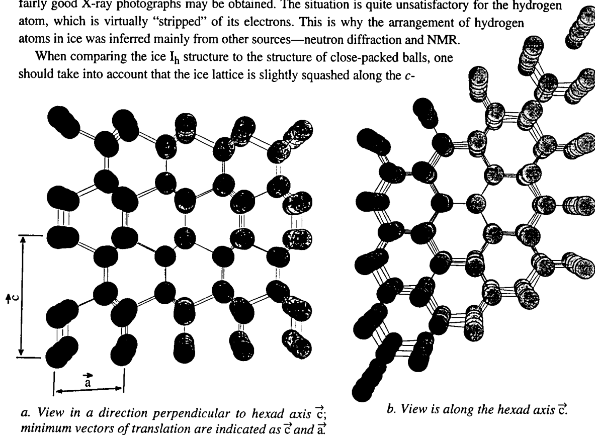
Figure 12. Positions of oxygen atoms in the ice I_h crystal. The shown size of atoms is not in real proportion to the inter atomic distance. Solid lines represent hydrogen bonds.
