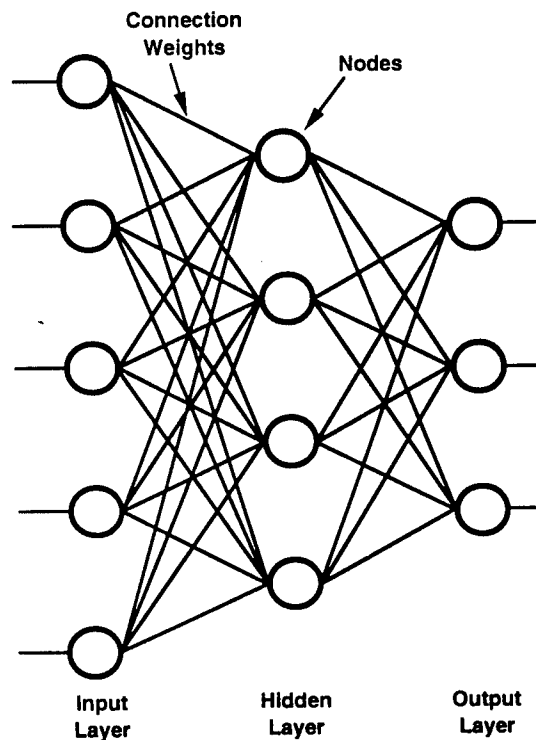
FIGURE 2.4-1. NEURAL NETWORK
