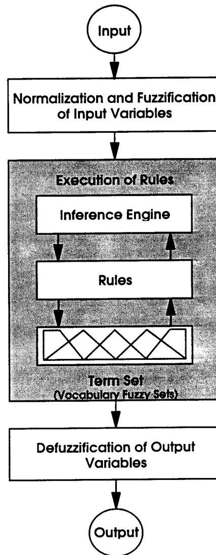
FIGURE 2.3-5. FUZZY CONTROLLER
