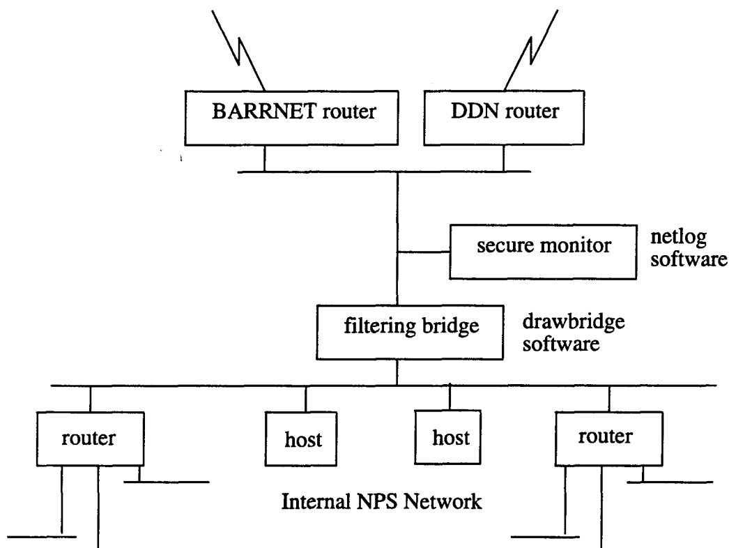
Figure 5: Firewall Overview
