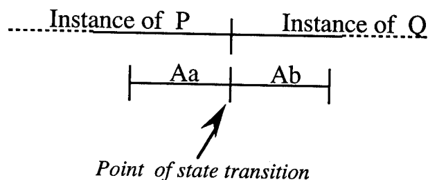
Figure 4-40. Interval Diagram for Figure 4-39
