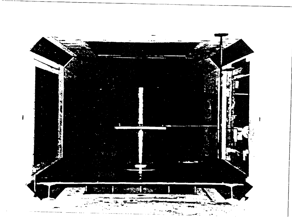
Figure 4.1 Balance Calibration Apparatus
