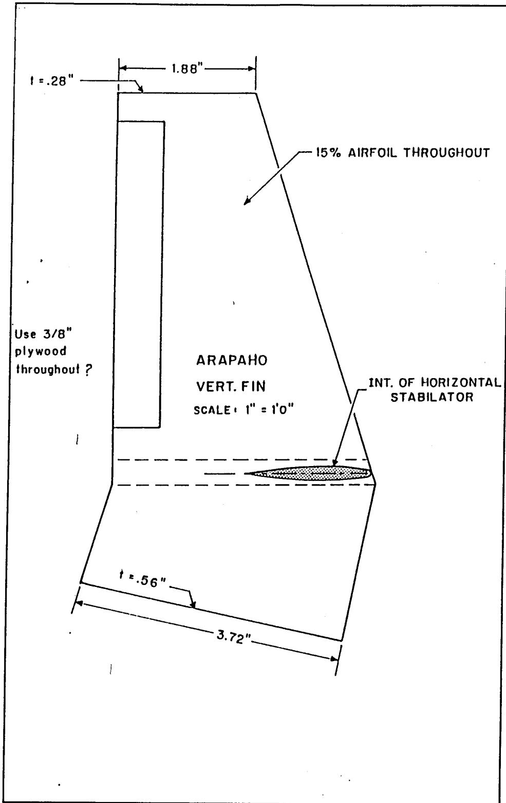
Figure 3.10 Vertical Tail
