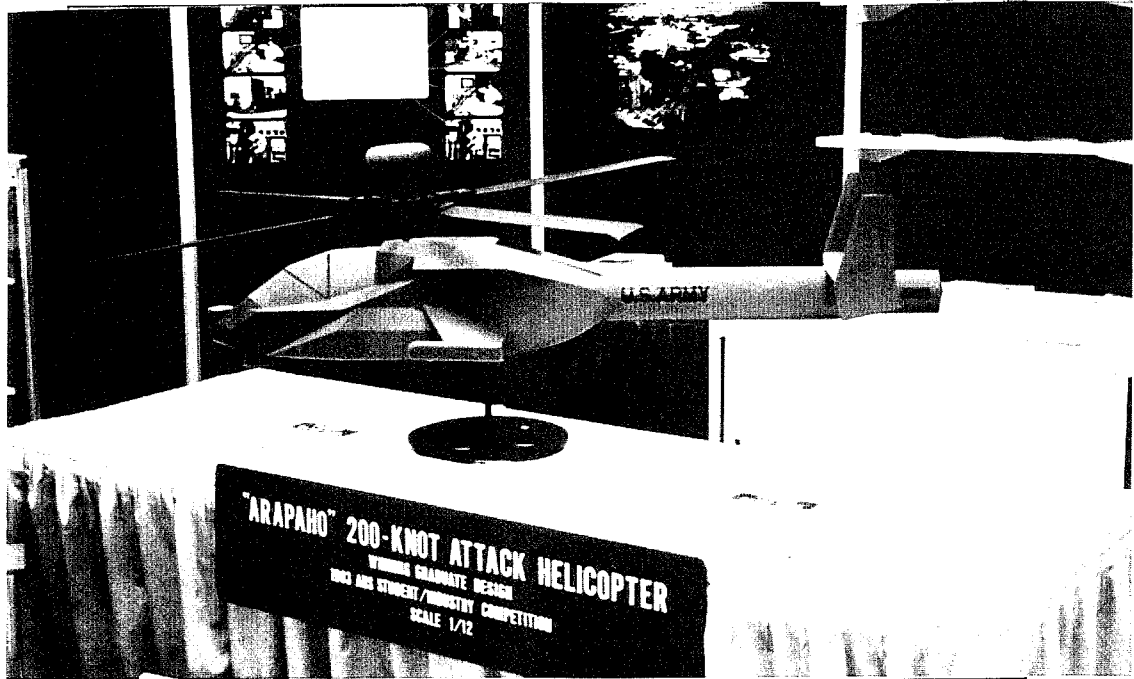
Figure 3.18 Completed Model
