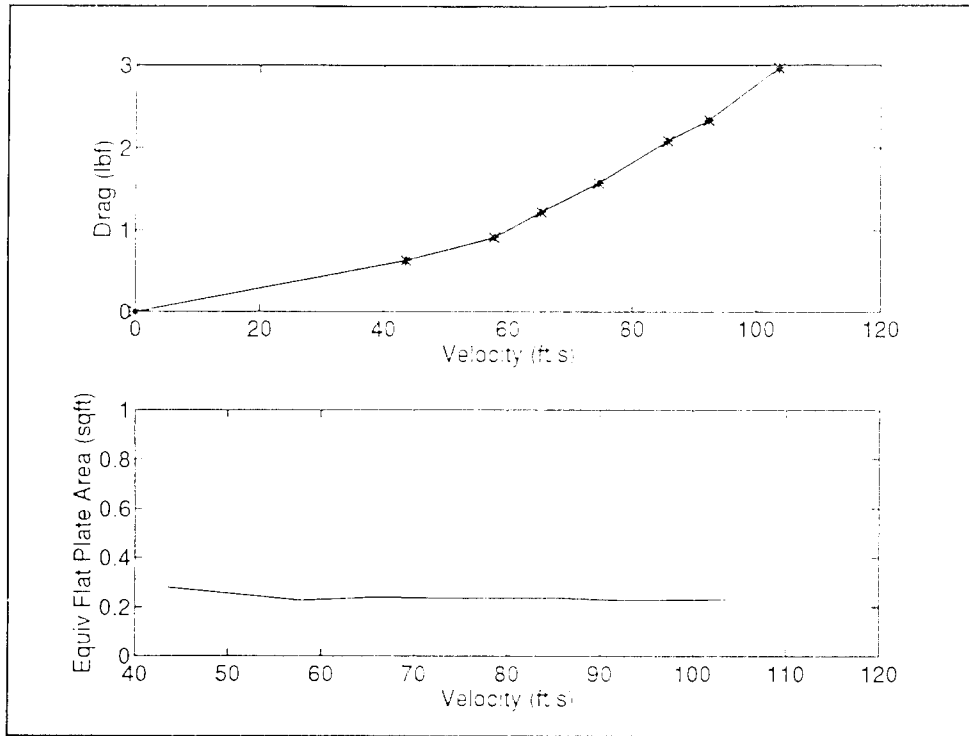
Figure 4.6 Drag and Equivalent Flat Plate Area, Basic Model - Run 1
