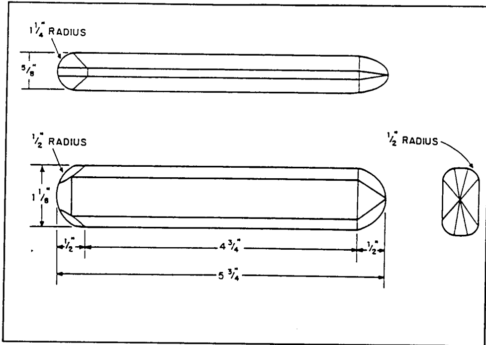
Figure 3.16 Stinger Pods
