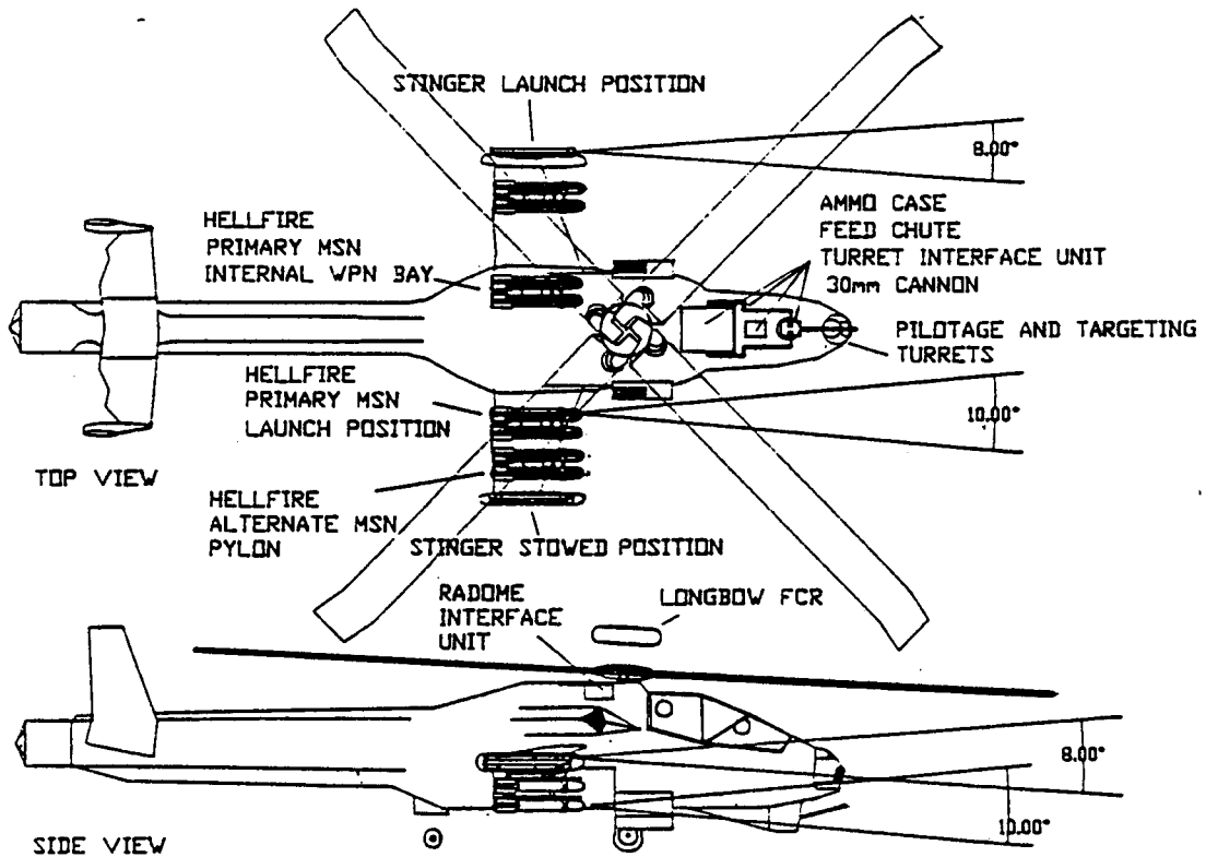
Figure 2.1 Arapaho Attack Helicopter
