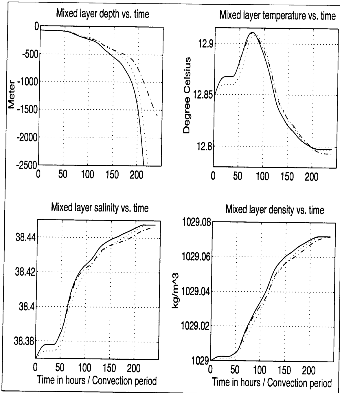
Figure 14. Kraus and Turner Simulation of the Variation of Mixed Layer Depth, Temperature, Salinity and Density with Time under Actual Windstress and Heat Flux using Adjusted Coefficients ( c_1=1, c_2=2 (.....) / c_1=2, c_2=1 (-.-.-) / c_1=2, c_2=2 (----)).
