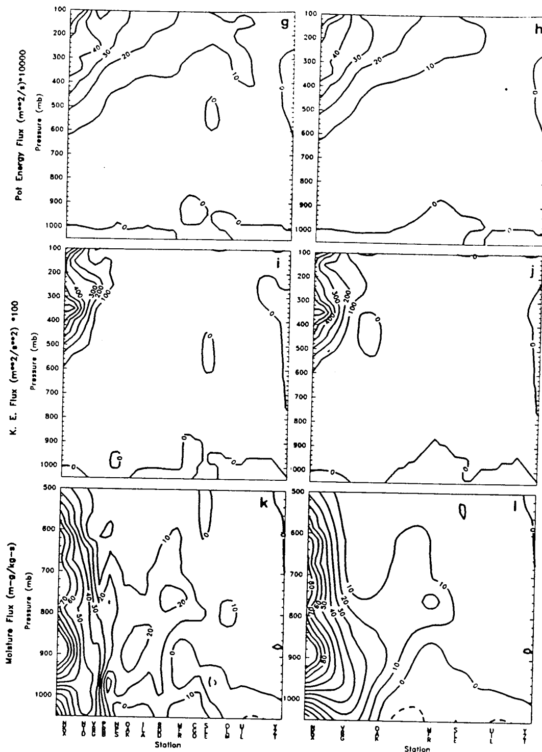
2100 UTC 15 Feb vertical cross sections for (g) ALL potential energy flux, (h) NWS potential energy flux, (i) ALL kinetic energy flux, (j) NWS kinetic energy flux, (k) ALL moisture flux, and (l) NWS moisture.
