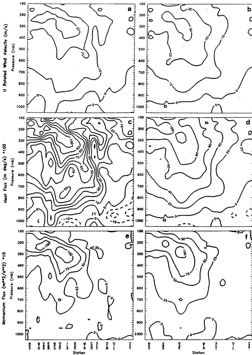
1800 UTC 14 Feb vertical cross sections for (a) ALL U_r flux, (b) NWS U_r flux, (c) ALL heat flux, (d) NWS heat flux, (e) ALL momentum flux, and (f) NWS momentum flux.
