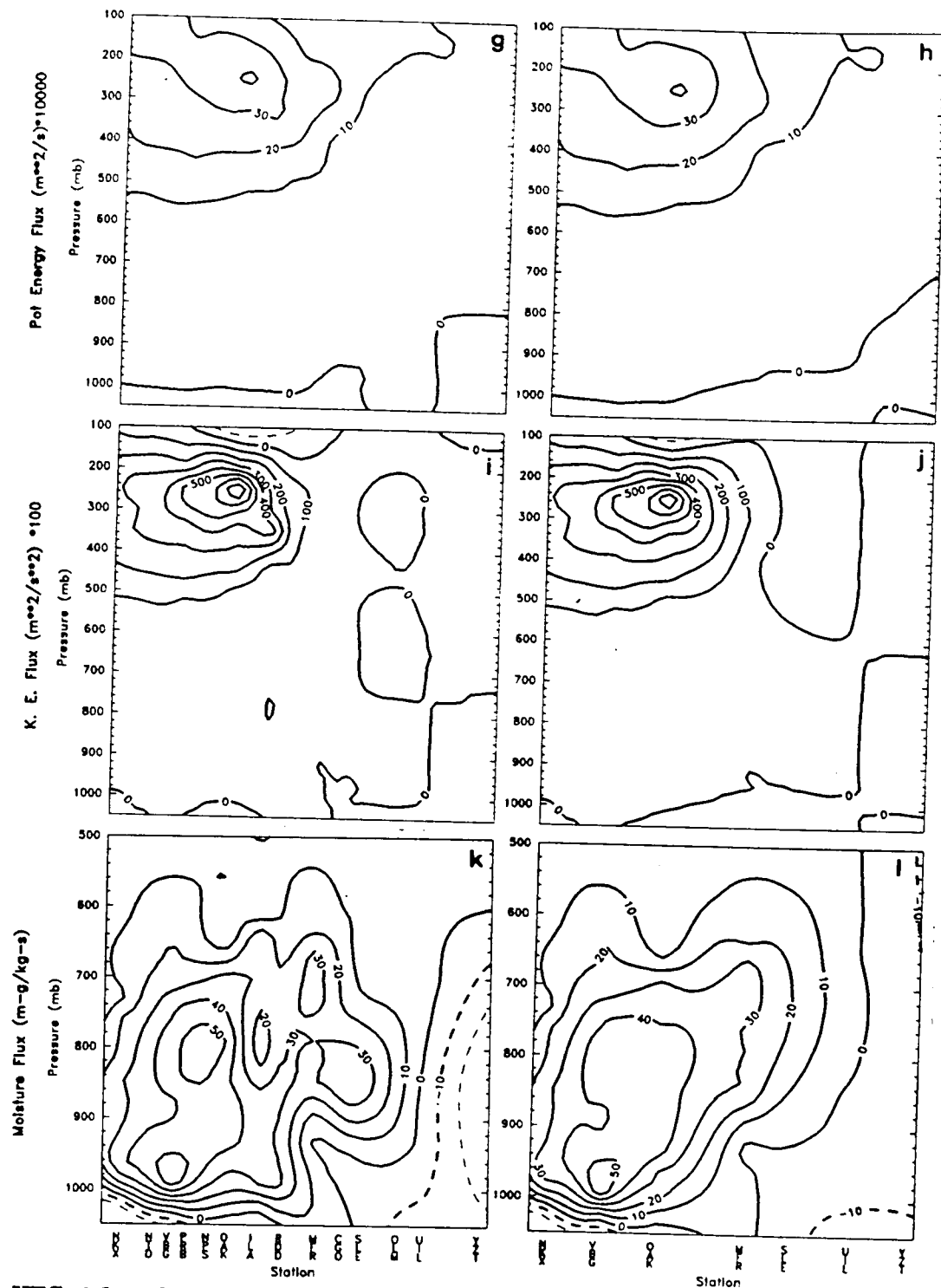
1500 UTC 16 Feb vertical cross sections for (g) ALL potential energy flux, (h) NWS potential energy flux, (i) ALL kinetic energy flux, (j) NWS kinetic energy flux, (k) ALL moisture flux, and (l) NWS moisture.
