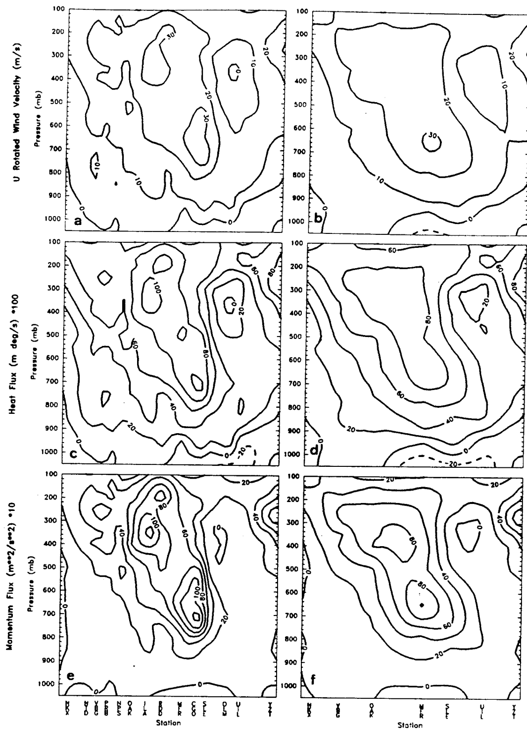
1200 UTC 20 Feb vertical cross sections for (a) ALL U_r flux, (b) NWS U_r flux, (c) ALL heat flux, (d) NWS heat flux, (e) ALL momentum flux, and (f) NWS momentum flux.
