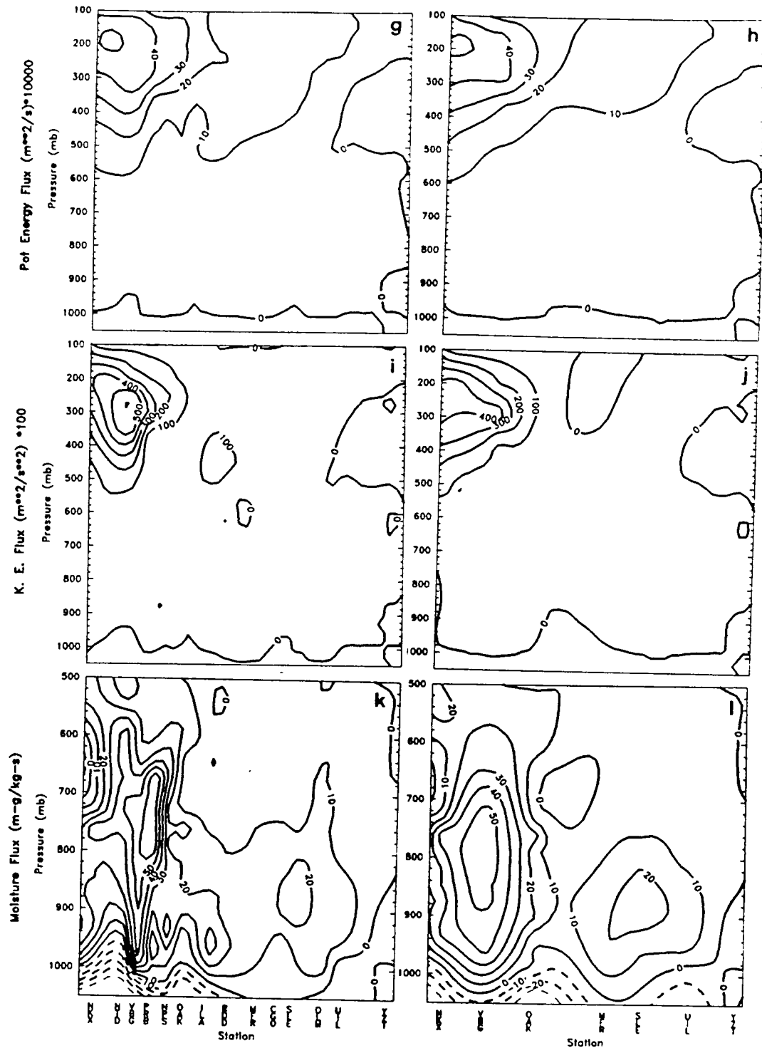
1200 UTC 15 Feb vertical cross sections for (g) ALL potential energy flux, (h) NWS potential energy flux, (i) ALL kinetic energy flux, (j) NWS kinetic energy flux, (k) ALL moisture flux, and (l) NWS moisture.
