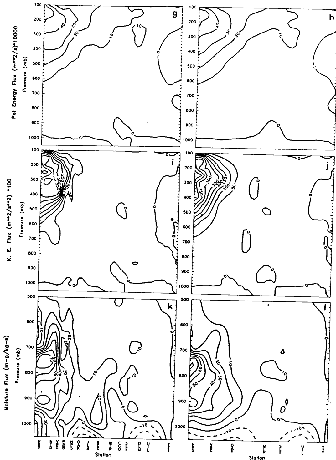
1800 UTC 15 Feb vertical cross sections for (g) ALL potential energy flux, (h) NWS potential energy flux, (i) ALL kinetic energy flux, (j) NWS kinetic energy flux, (k) ALL moisture flux, and (l) NWS moisture.
