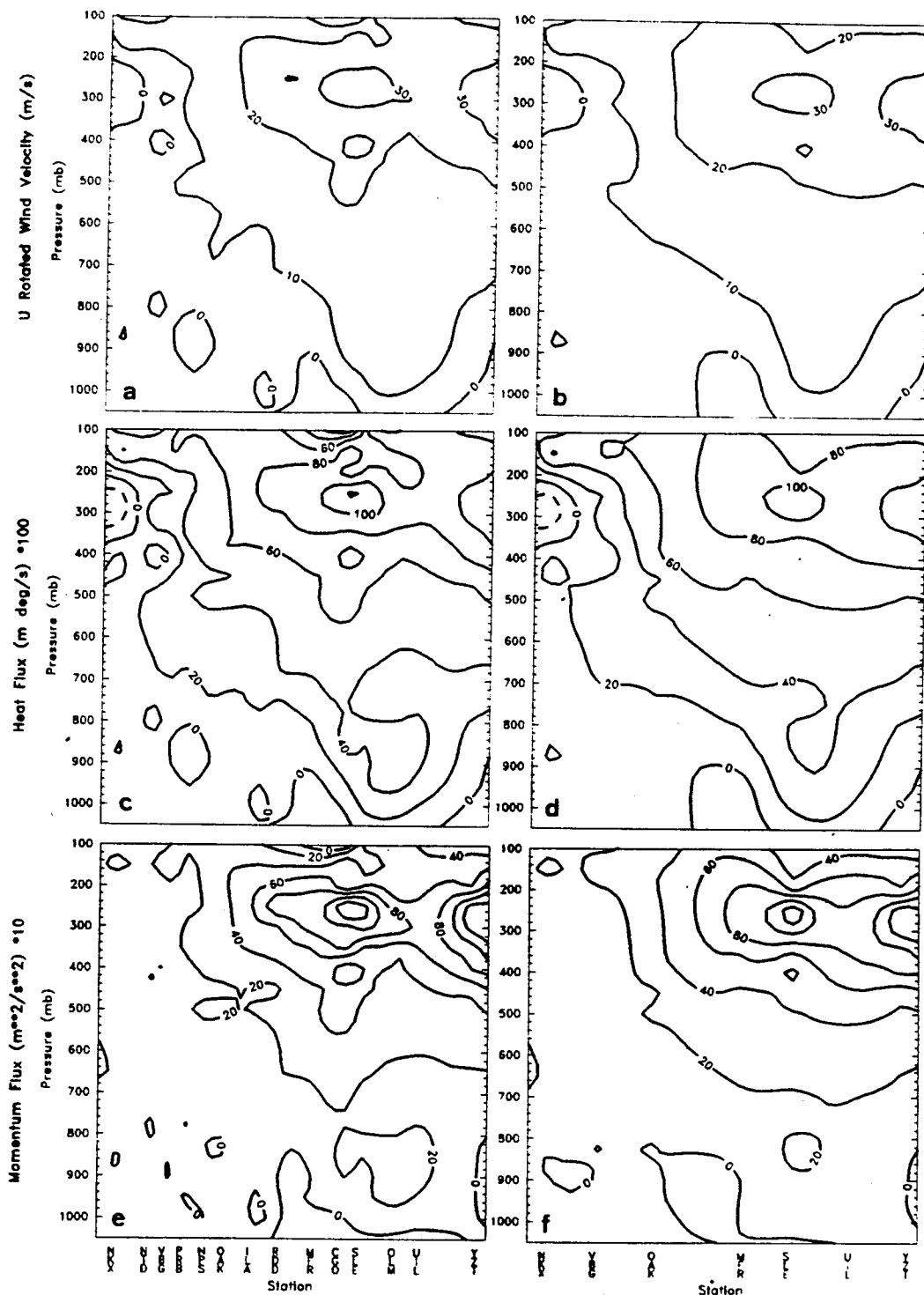
0000 UTC 21 Feb vertical cross sections for (a) ALL U_r flux, (b) NWS U_r flux, (c) ALL heat flux, (d) NWS heat flux, (e) ALL momentum flux, and (f) NWS momentum flux.
