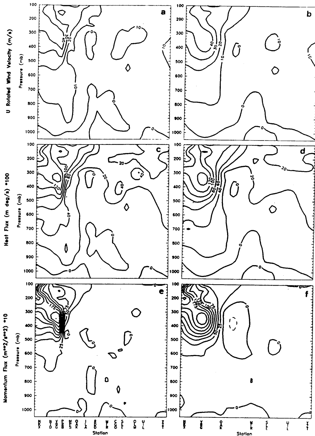
0900 UTC 6 Mar Vertical cross sections for (a) ALL U_r flux, (b) NWS U_r flux, (c) ALL heat flux, (d) NWS heat flux, (e) ALL momentum flux, and (f) NWS momentum flux.
