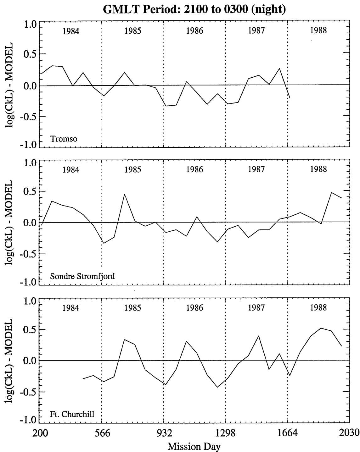
Figure 6: Variation of the residual \log(C_k L) as a function of days since the launch of HiLat at Tromso (top plot), Sondre Stromfjord (middle plot), and Ft. Churchill (bottom plot) for the night sector (2100 to 0300 GMLT).
