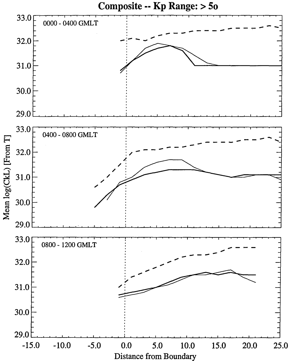
Figure 57: Comparison of WBMOD Version 12.02 (heavy dashed line) and SCINTMOD Version 1.0 (heavy solid line) to composite observations of \log(C_k L) (light solid line) for all SSN and K_p \geq 5.0 .
