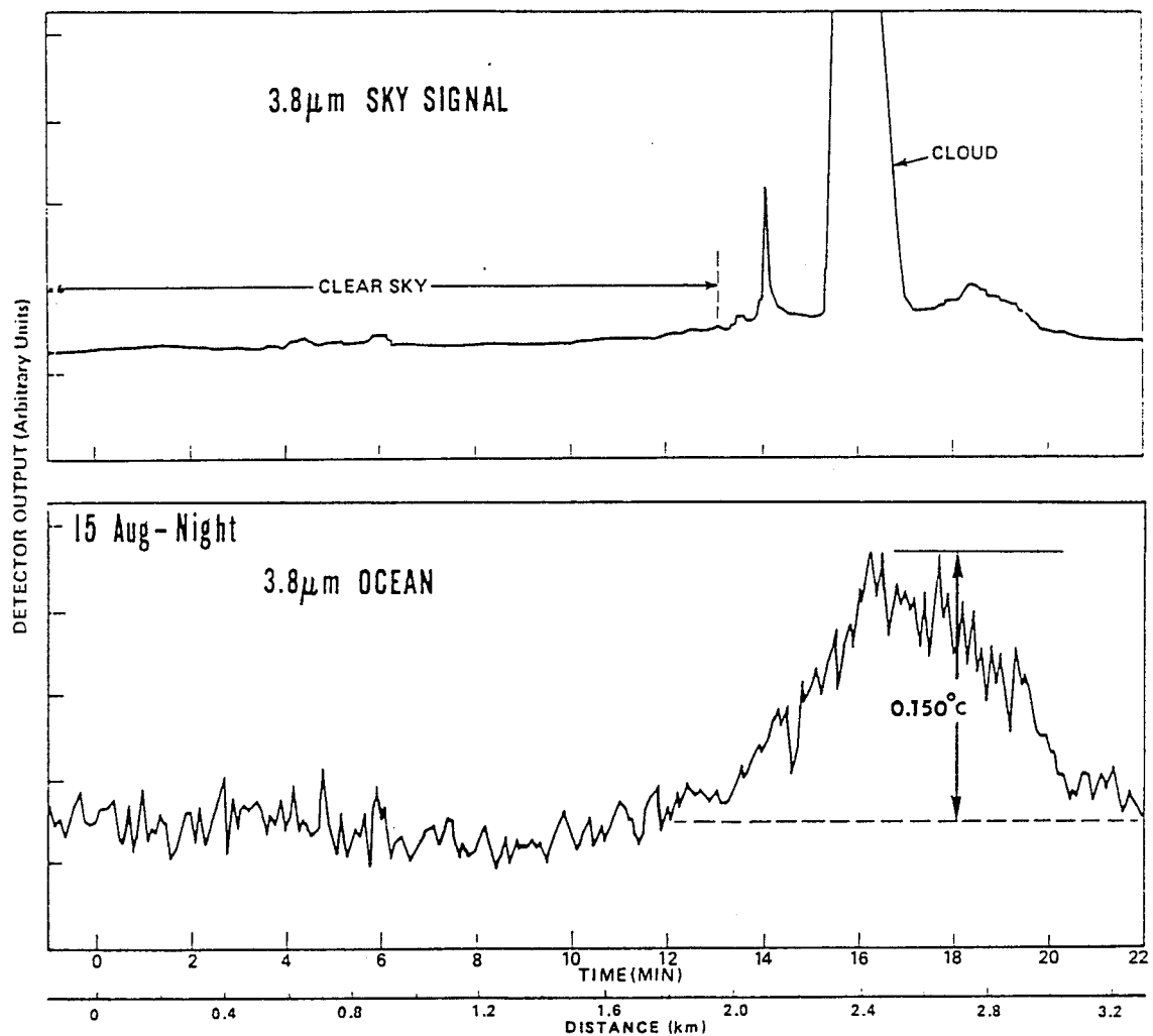
Figure 3.24 Data segment from the 3.8 \mu m channel on August 15, 1973 at 20° incidence angle. Each point plotted represents an average over 4.5 seconds with the vessel underway at 3.5 m/s (from Gasparovic et al. , 1974).
