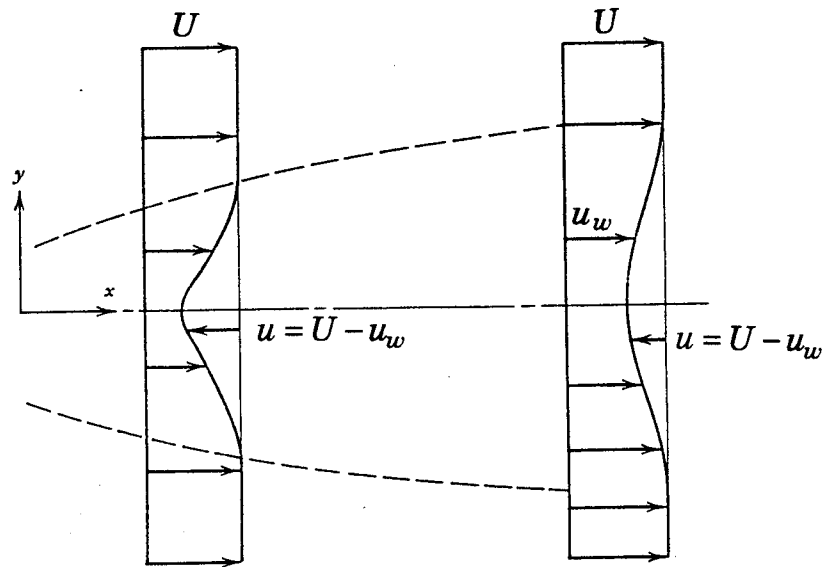
Figure 4.5 Laminar wake of a bluff body, i.e. circular cylinder (from Panton, 1984).
