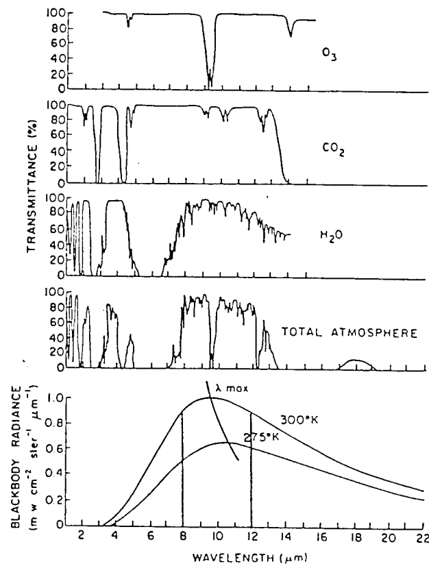
Figure 3.11 Upper curves: Transmission spectra of the three principal absorbing atmospheric gases (ozone, carbon dioxide, and water vapor) and the whole atmosphere at vertical incidence for infrared wavelengths.
