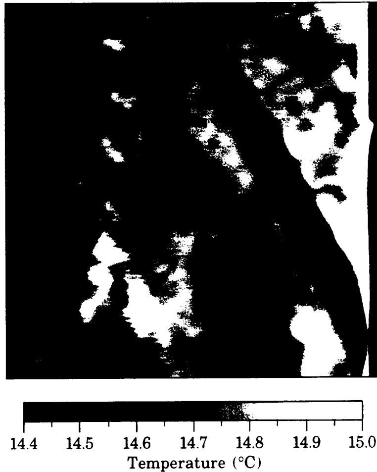
Figure 5.8 Infrared image of the serpentine nature of the wakes emanating from the instrument cables when the waves and current are not aligned. The wakes are located in the upper left corner. A guy wire runs diagonal through the image. Hints of boom reflection appear below the wakes.
