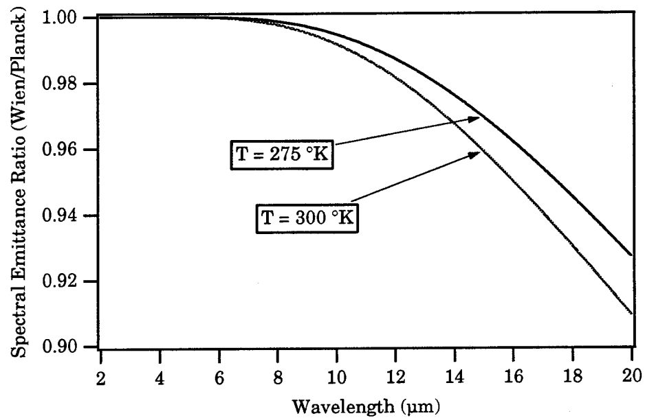
Figure 3.3b Deviation from Planck's blackbody radiation law according to Wien's approximation.
