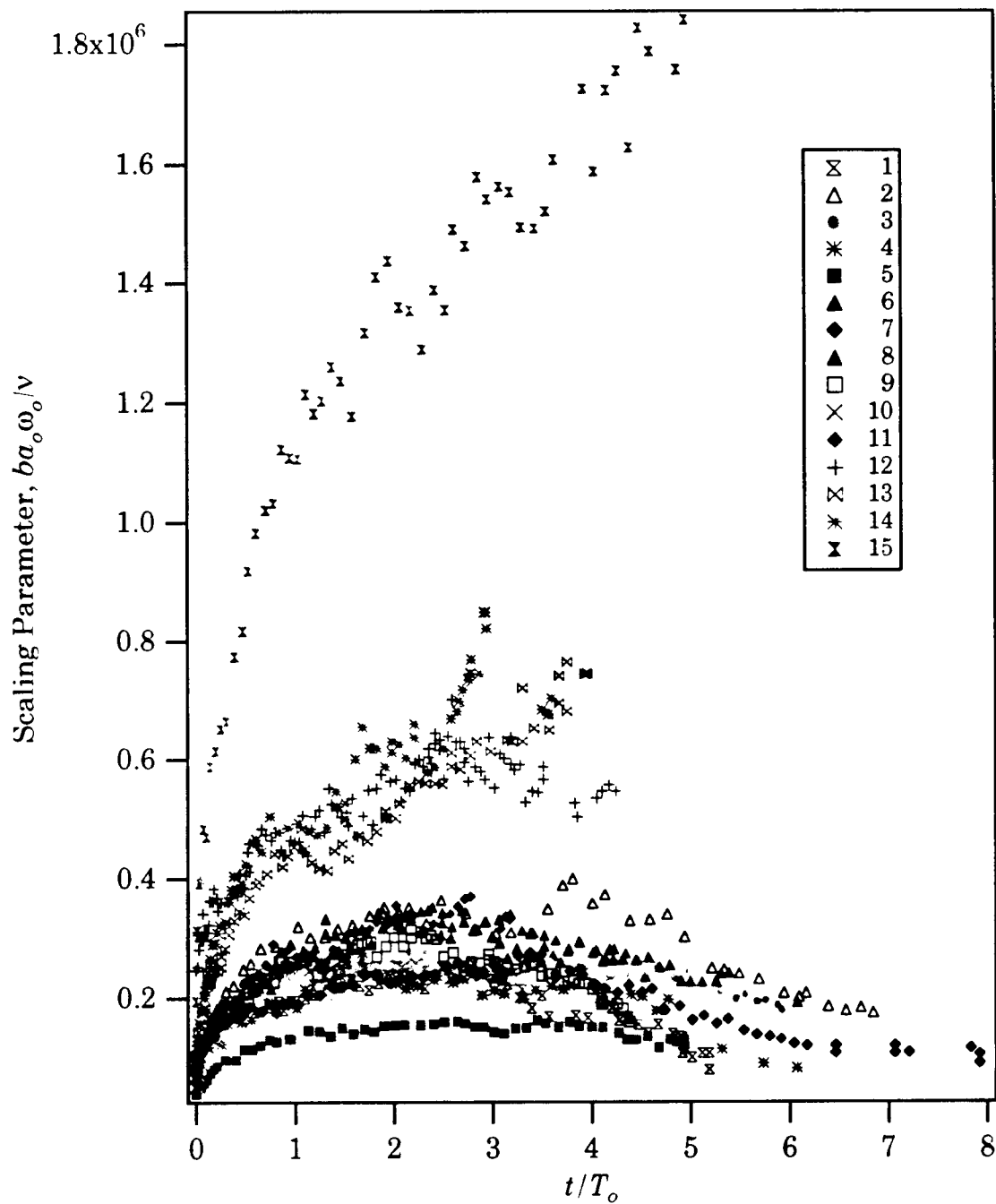
Figure 5.18 Scaling analysis of the the 15 individual patches produced by the swell. Both t/T_o and ba_o\omega_o/\nu separate out into three distinct regions according to the Re_w . The regions follow from bottom to top as low, mid, and high range Re_w .
