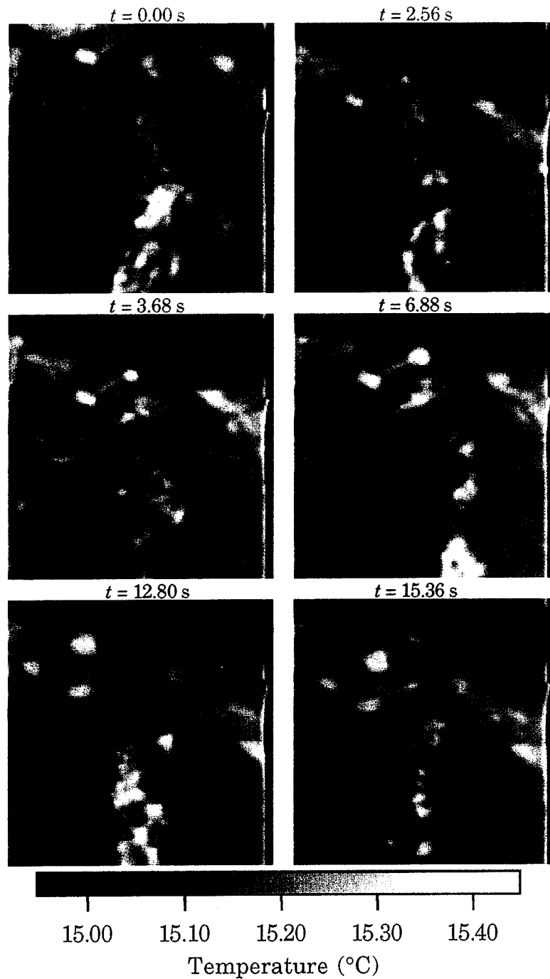
Figure 5.10 Time series of infrared images depicting the ordered wakes emanating from the surface-piercing cables under low wind conditions when the swell waves propagate in the direction of the current. The long slender wakes develop by the superposition of the crest of the swell and the current velocities. The patches form when the velocity in the trough counteracts the current. The cable diameter is 1 cm while the patches are on the order of 1 m.
