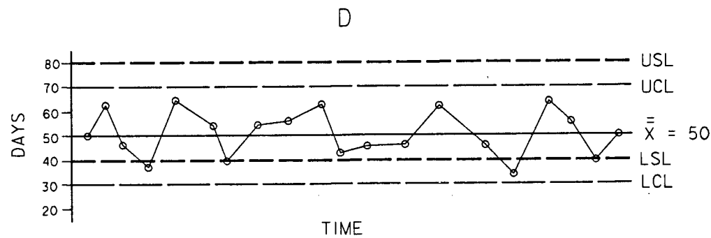
Figure 33 Process Capability Analysis
