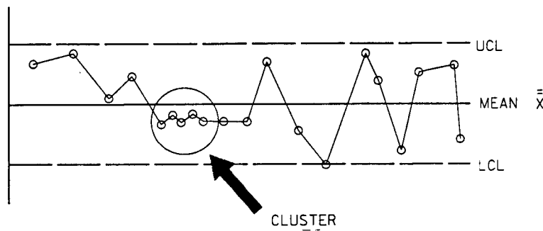
Figure 17 Out of Control Patterns for X and R Charts
