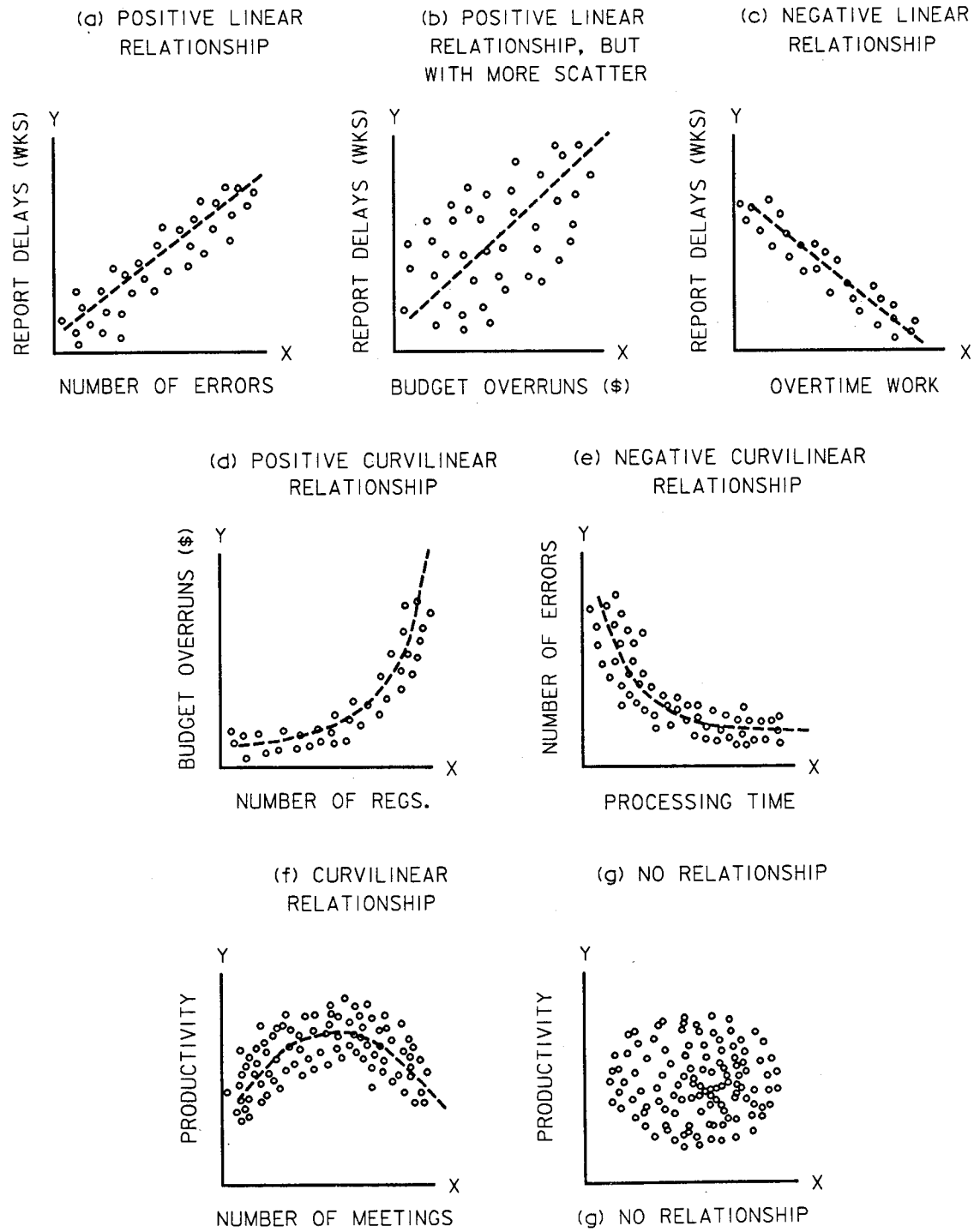
Figure 26 Examples of Scatter Diagrams
