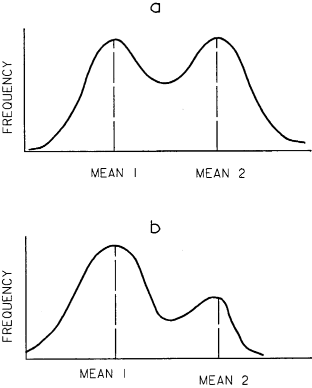
Figure 7 Shapes of Distributions
