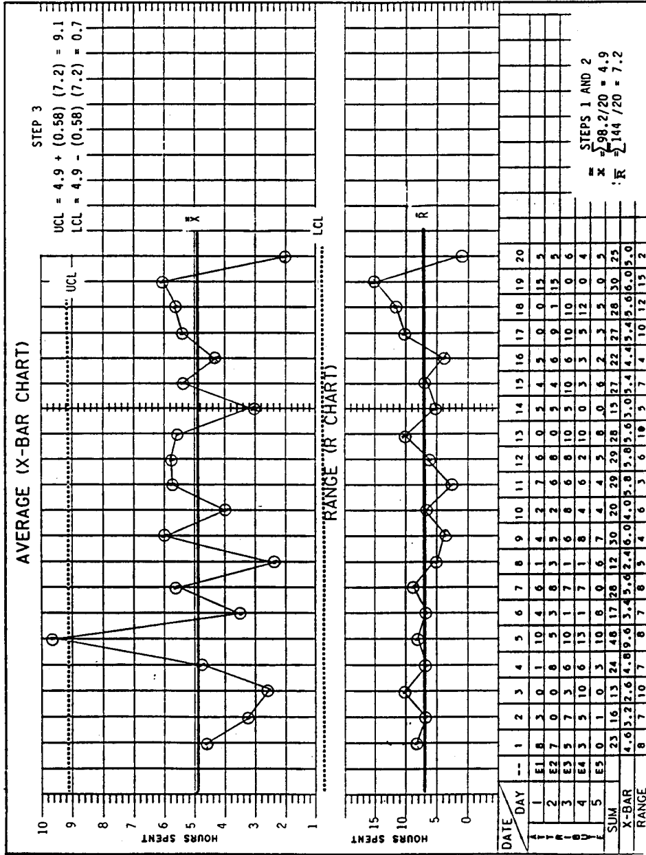
Figure 23 Shewhart Control Chart
