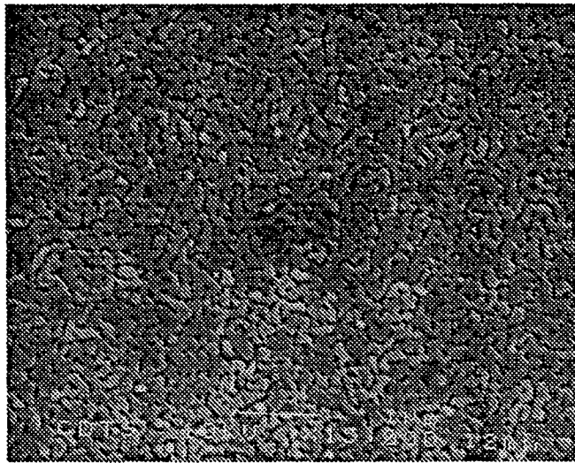
Figure 7. SEM micrograph of 1000 Å thick CaRuO 3 film on LaAlO 3 substrate (15 kX magnification).
