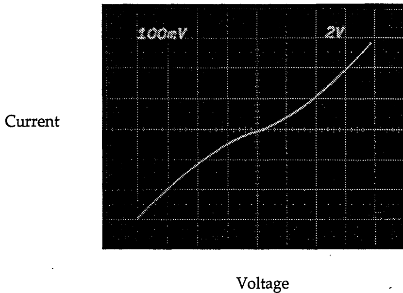
Figure 8. Current-voltage data at 77 K for YBCO/CaRuO 3 /YBCO SNS junction made using SSMOCVD. Plot scales are 100 μA/division vertical and 2 V/division horizontal.
