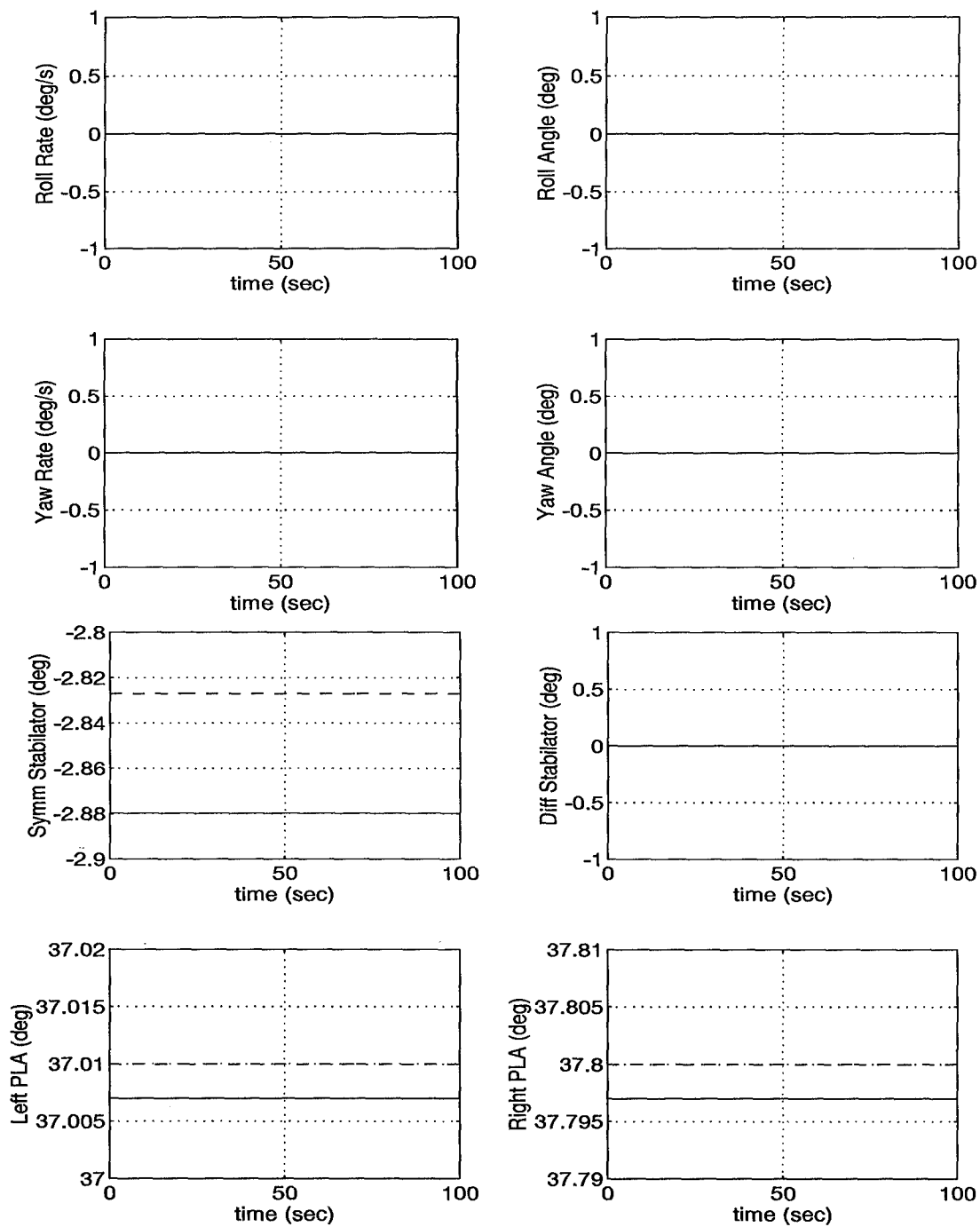
Figure B.2: Flight Point 1—Aircraft Responses to Initial Conditions Set at Trim Values: MATLAB (solid line) and Genesis (dashed line).
