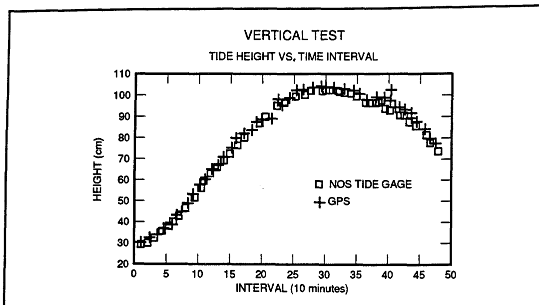
Figure 5. Vertical test results (□ represents NOS tide gage; + represents GPS)
