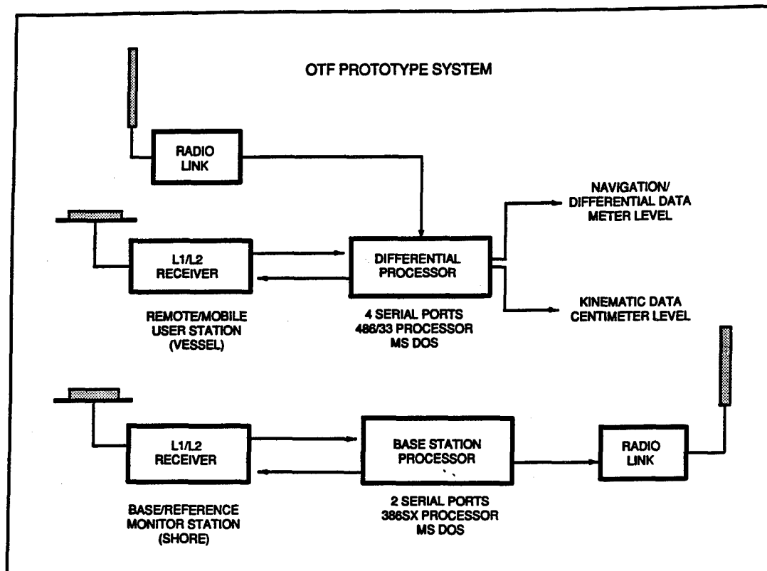
Figure 1. Block diagram of OTF prototype system
