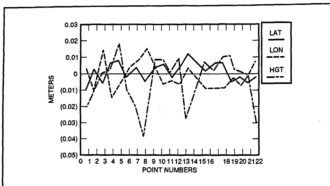
Figure 4. Kinematic land test results
