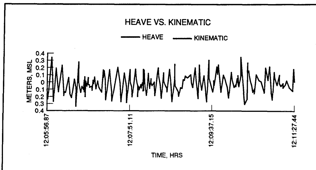
Figure 6. KOTF data compared to heave compensator data
