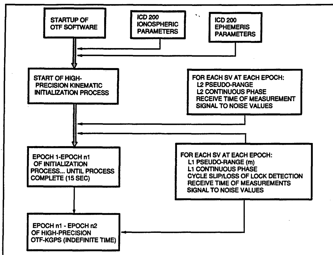
Figure 2. Schematic of information flow required by OTF system
