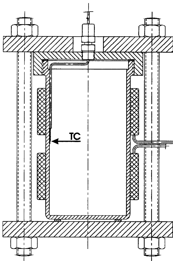
Figure 3 The TNO-PML SCB test
