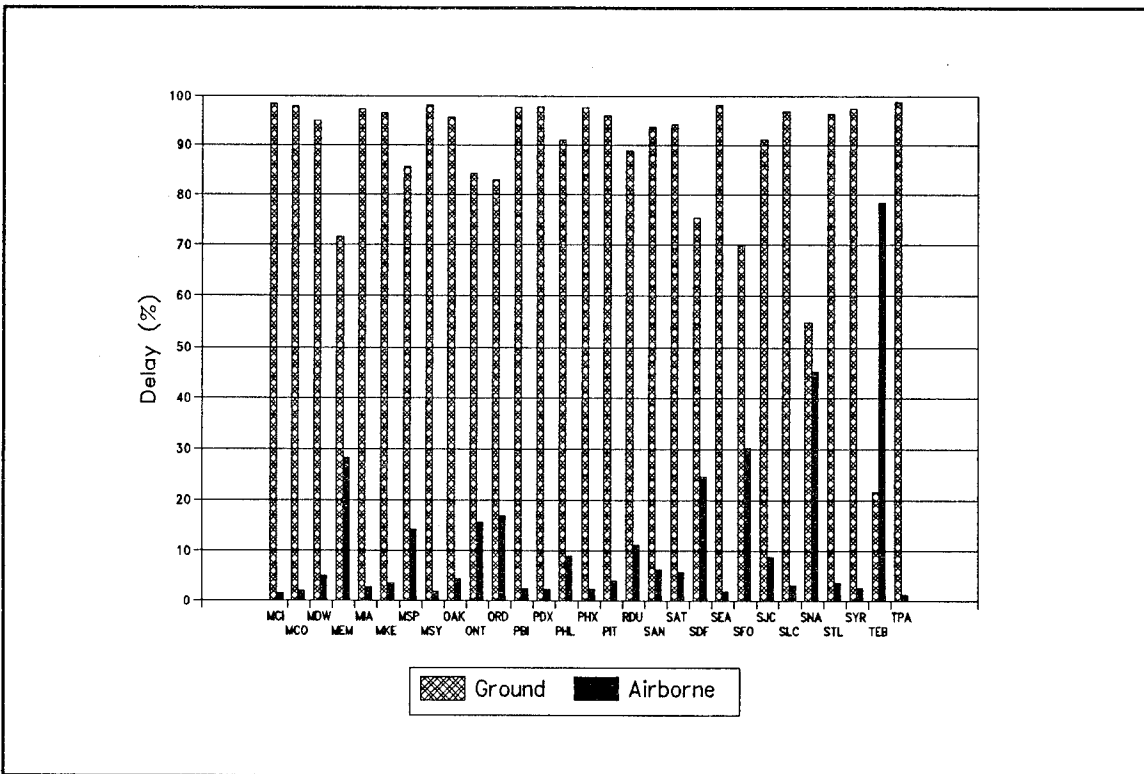
FIGURE 16. GROUND DELAY VS AIRBORNE DELAY YEAR 2005 (2 OF 2)
