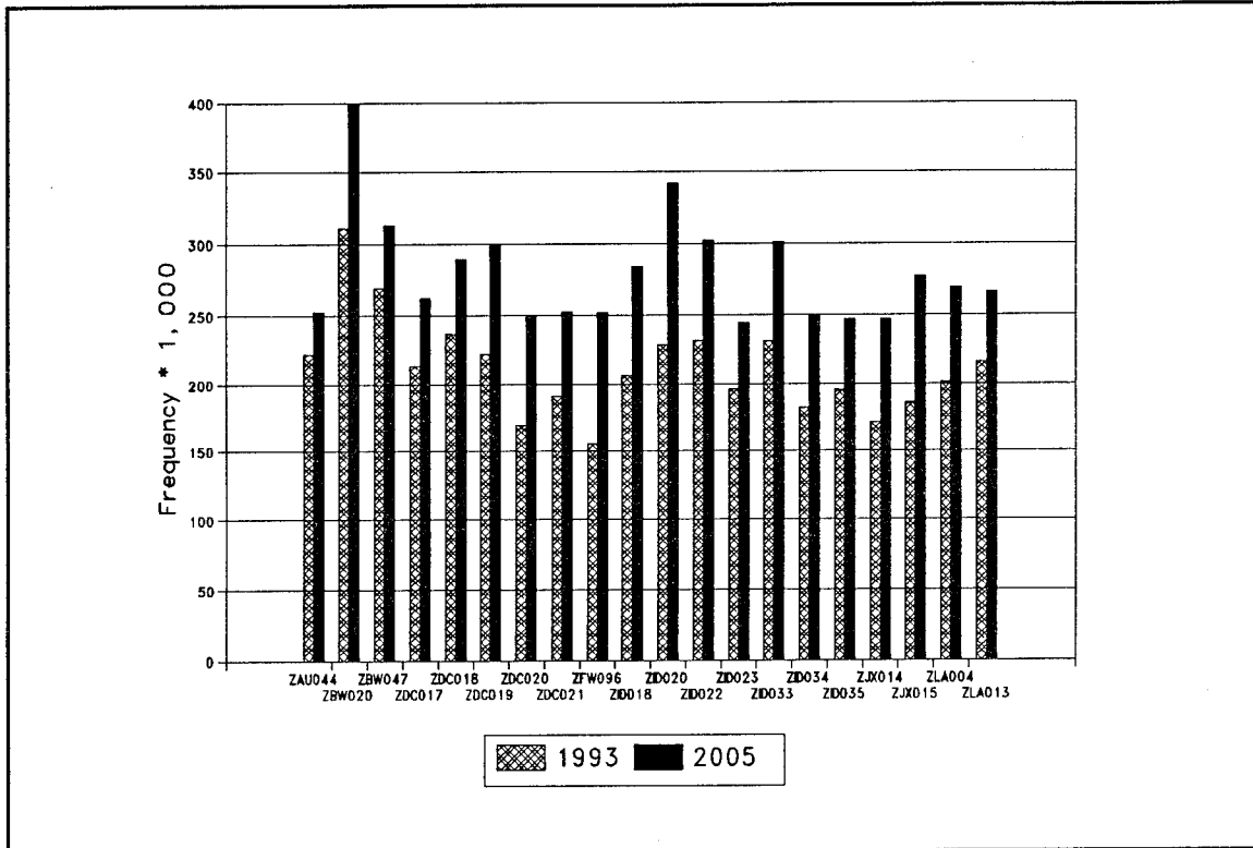
FIGURE 18. ANNUAL SECTOR THROUGHPUT (1 OF 2)
