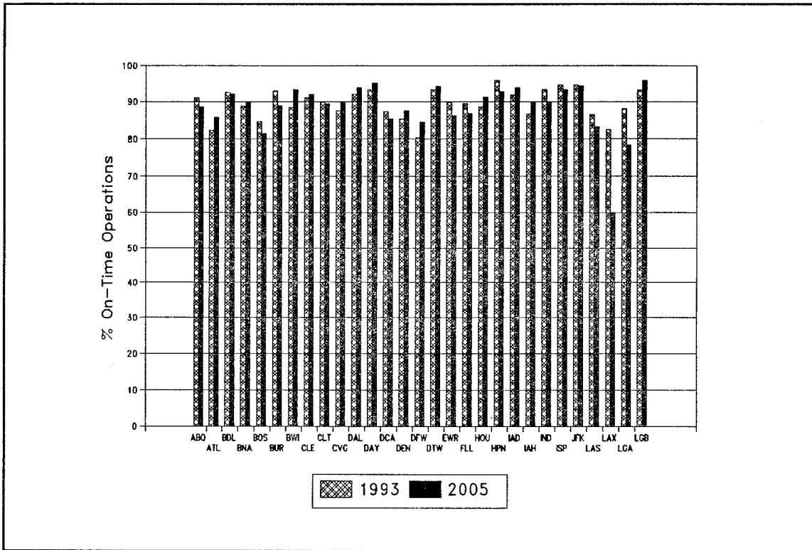
FIGURE 14. OPERATIONS WITH PASSENGER DELAY UNDER 15 MINUTES (1 OF 2)
