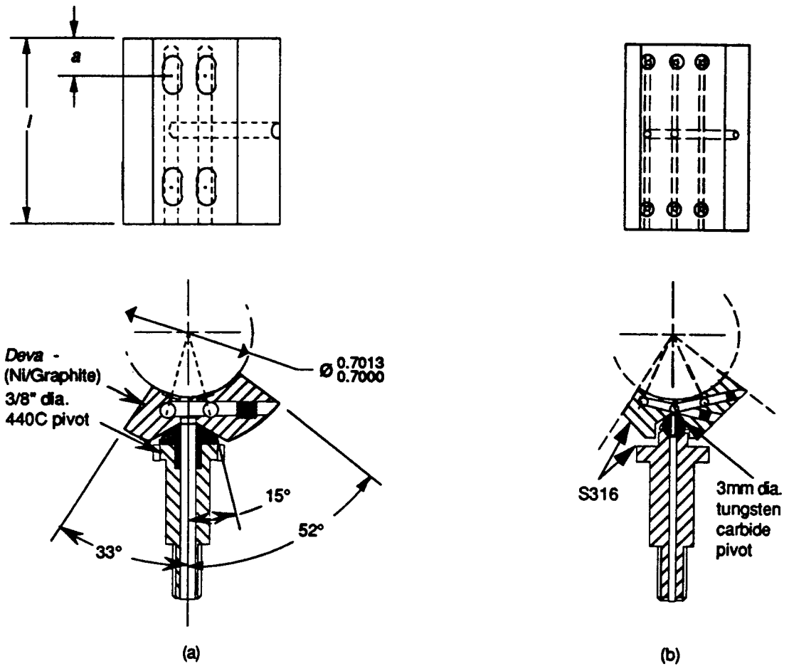
Figure 2.16 Final (a) and Prototype (b) Hybrid Pad Sectioned at Middle Station
