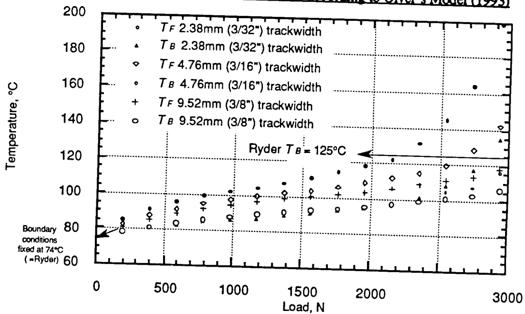
Figure 2.3 Thermal Behaviour of Mini-Disc according to Olver's Model (1993)
