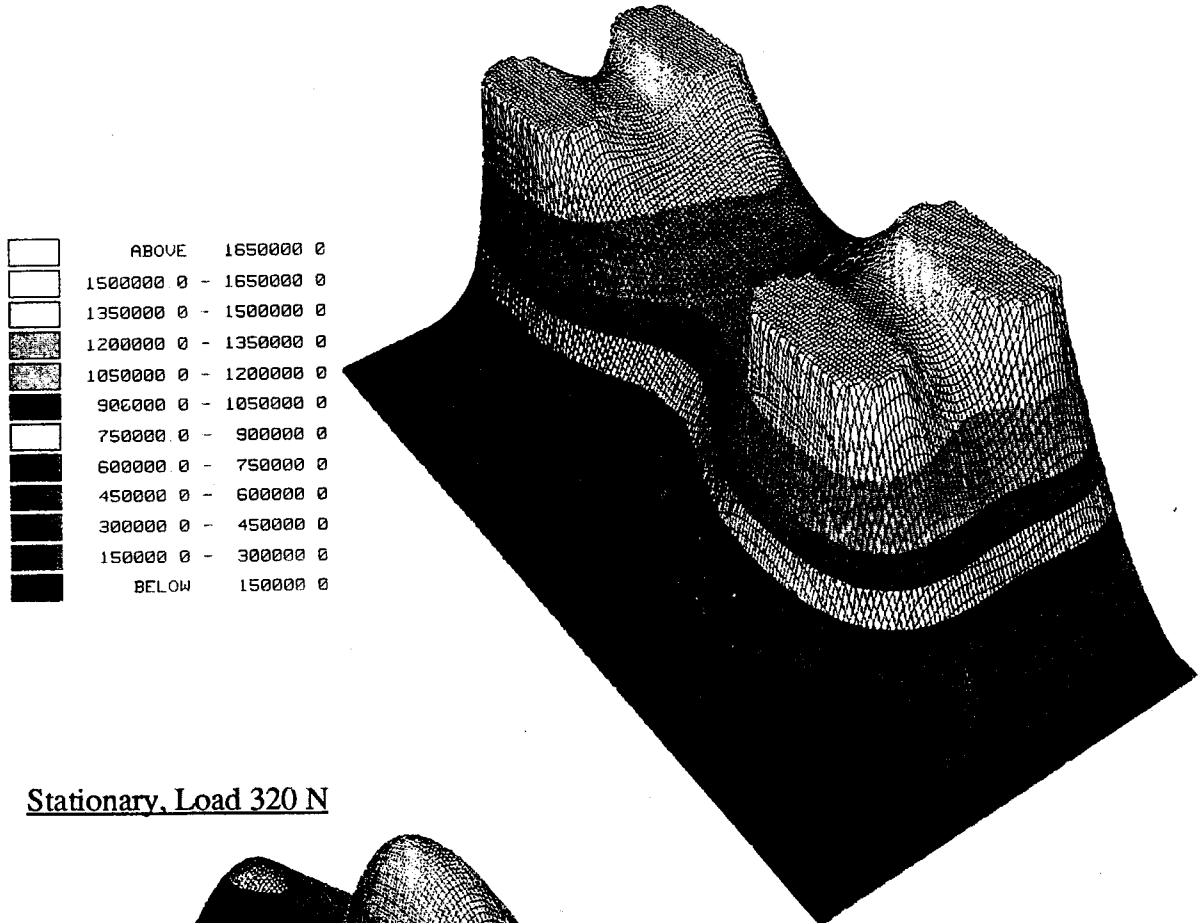
Figure 2.14 Hybrid Pad Performance, Predicted Isoviscous Pressure Profiles
