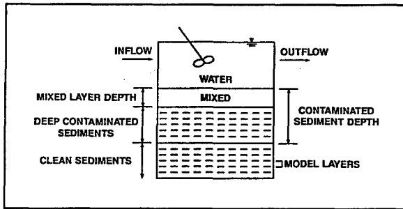
Figure 1. Physical configuration of RECOVERY
