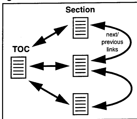
Figure 5-3: TOC-Outline Structure
