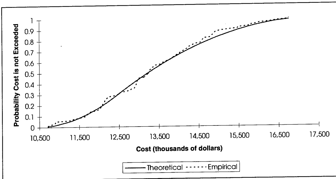
Figure 2. Theoretical and Empirical Distributions of Program Support Cost (100 Simulations)
