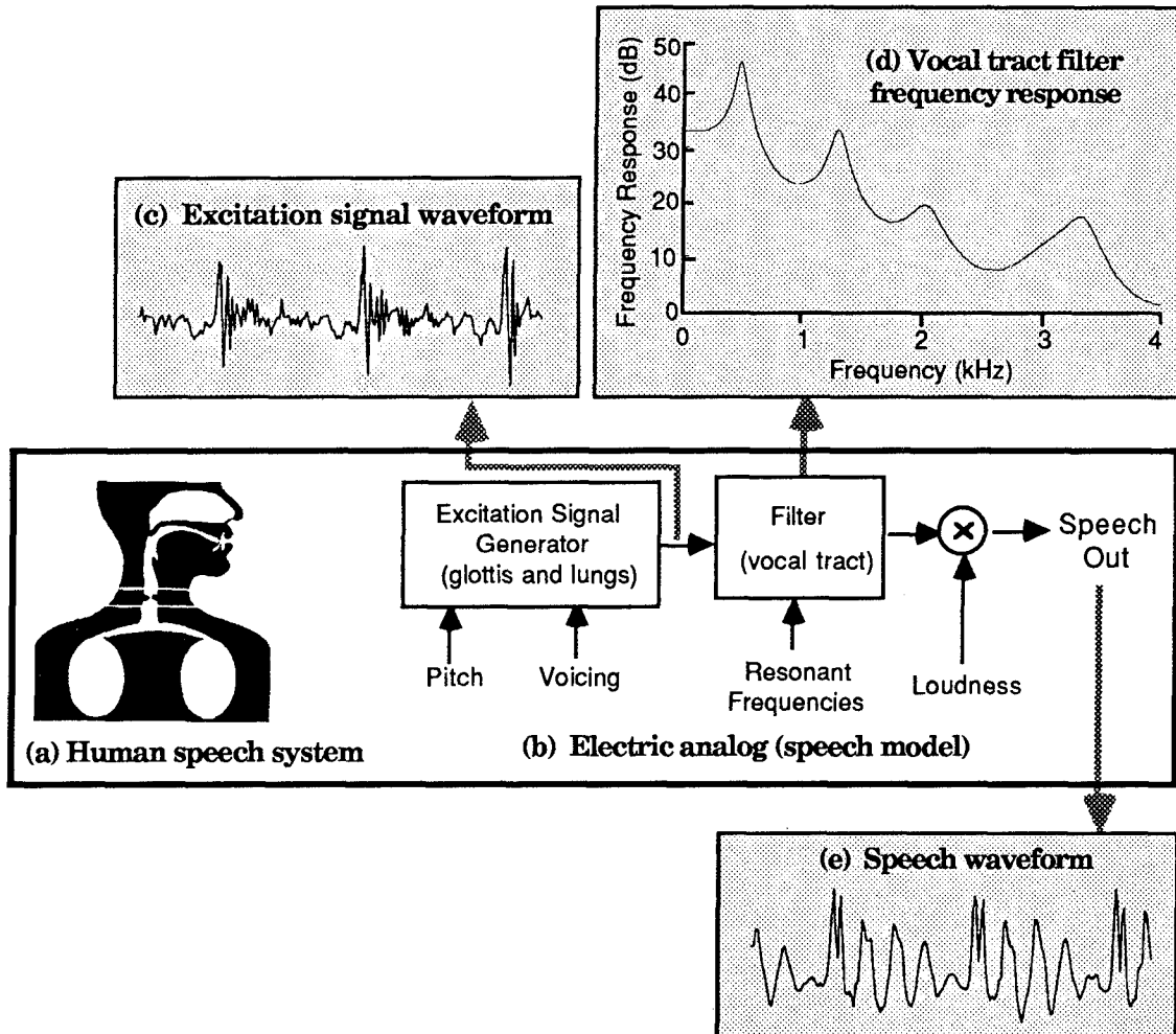
Fig. 1 — Generic speech model based on the human speech production mechanism. The speech waveform (Fig. 1(e)) is the only quantity that is available. The vocal tract filter response (Fig. 1(d)) must be estimated from the speech waveform. The excitation signal (Fig. 1(c)) is modeled by either a pulse train (to generate vowels) or random noise (to generate consonants). The use of such a simple signal enables us to control the pitch period, utterance rate, and resonant frequencies independently.
