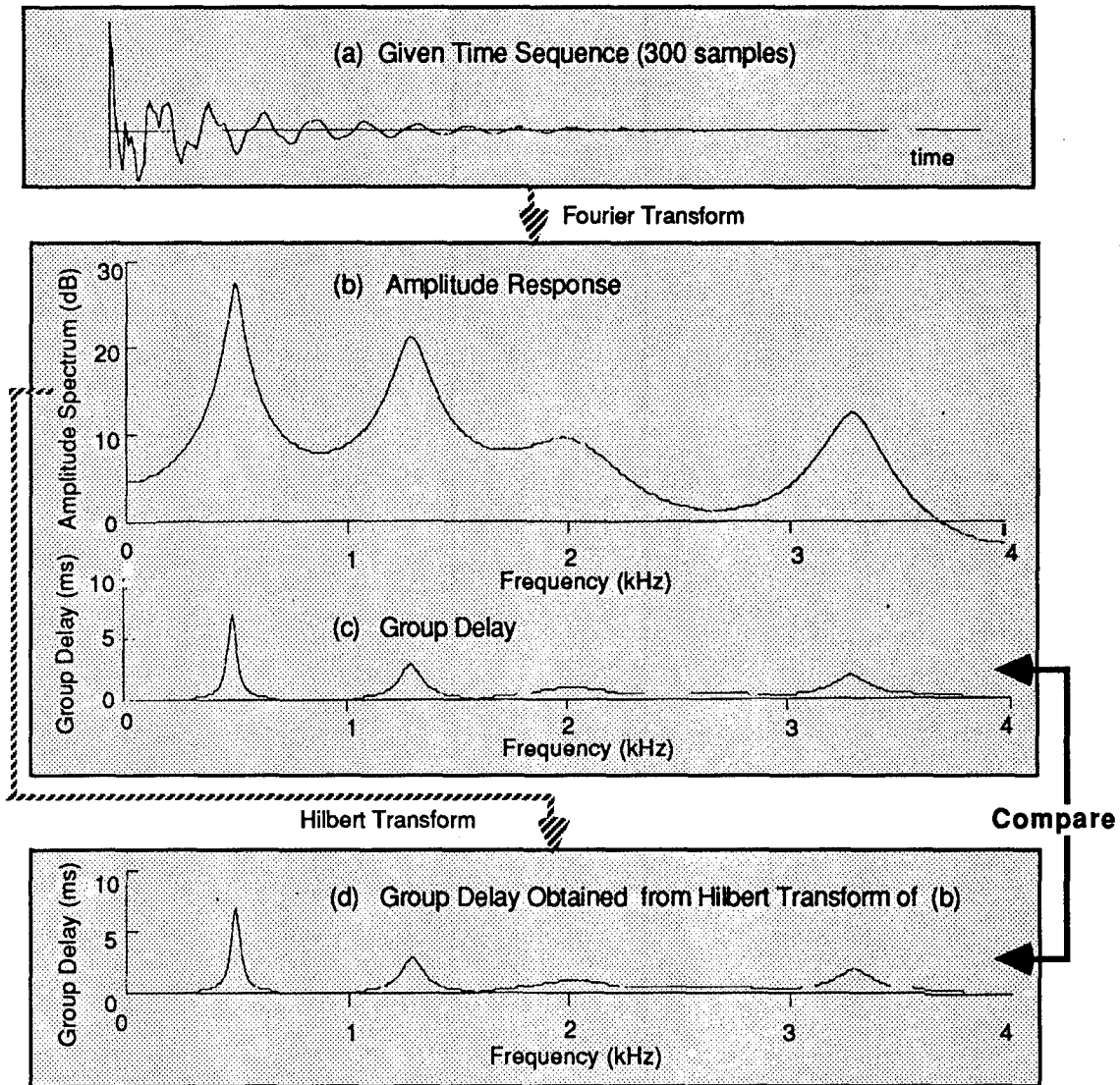
Fig. 22 — Comparison of two group delays. Time sequence (Fig. 22(a)) generates both the amplitude spectrum (Fig. 22(b)) and group delay (Fig. 22(c)) via the Fourier transform. Since the time sequence is causal (i.e., x[n] = 0 for n < 0 ), the Hilbert transform of the amplitude spectrum provides the group delay (Fig. 22(d)). The similarity between Figs. 22(c) and Fig. 22(d) is excellent. This is the reason why the phase spectrum of the pitch waveform need not be encoded.
