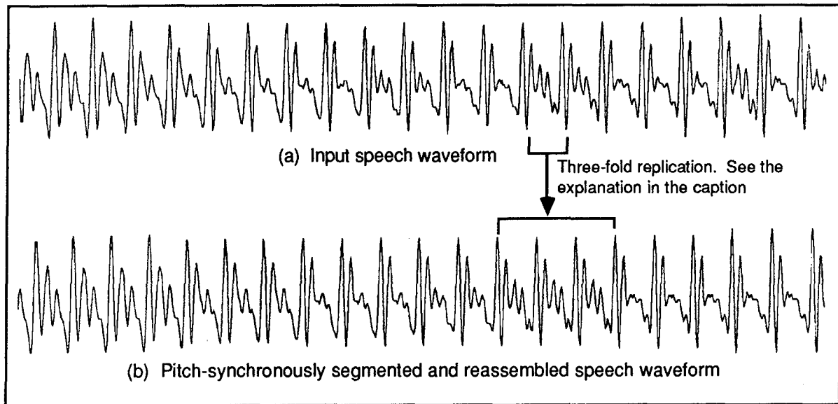
Fig. 9 — Input and output speech waveforms. Comparison of these two waveforms shows that pitch-synchronous segmentation and concatenation produces a nearly flawless result. Output speech sounds almost as good as input speech. This is an example from a high-pitched voice, pitch period is 44 and frame size is 120. Thus, each segmented speech waveform is repeated approximately three times per frame, on the average.
