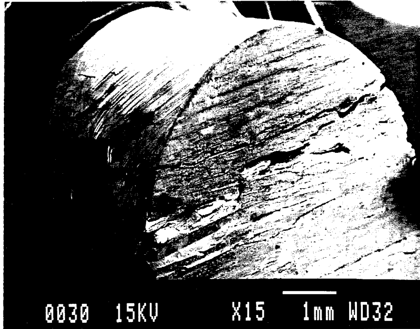
Figure 36a. [110] crystal - slip traces and cleavage.
