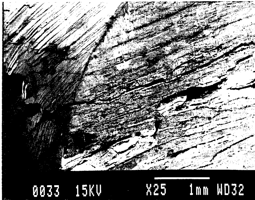
Figure 36b. [110] crystal - slip traces and cleavage.
