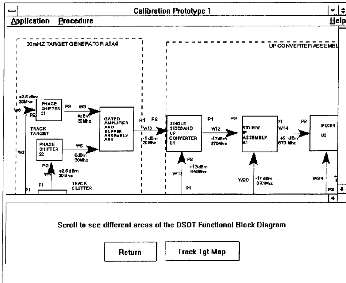
Figure 9. Example of diagram in MK 92 Mod 2 MAES (some quality has been lost in importing this graphic)
