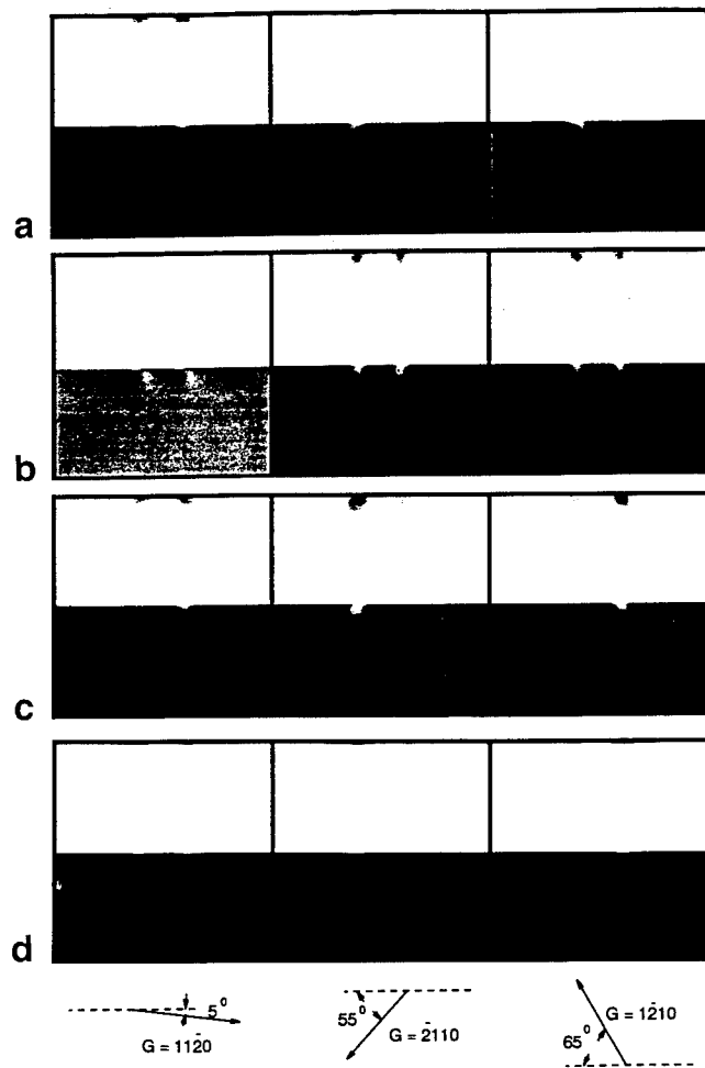
Fig. 11 Bright field (top) and dark field (bottom) diffraction contrast image simulations of the finite element model under different diffraction conditions, w=1.0 and t=1.3 \zeta_0 : (a) concentrated shear load; (b) concentrated normal load; (c) both shear and normal; (d) surface contraction
