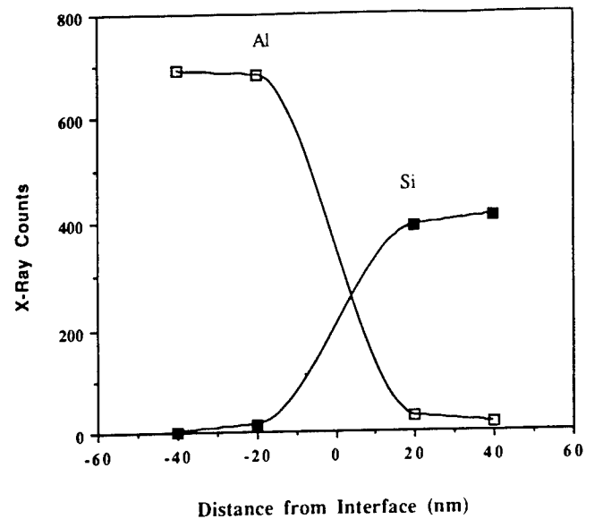
Fig. 2 Linescan profile across the interface. This shows the interface to be very stable and free of any segregation
