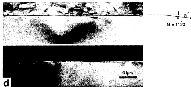
Fig. 10 TEM micrographs of clean interface between the single crystal \text{Al}_2\text{O}_3 filament and NiAl matrix, after 10 thermal cycles: (a) the inhomogeneous diffraction contrast observed along the interface on the \text{Al}_2\text{O}_3 filament side; (b)–(d) bright (top) and dark (bottom) field images of the interface with different operating diffractions, t = 1.3 \xi_0 with G = \{1120\}
