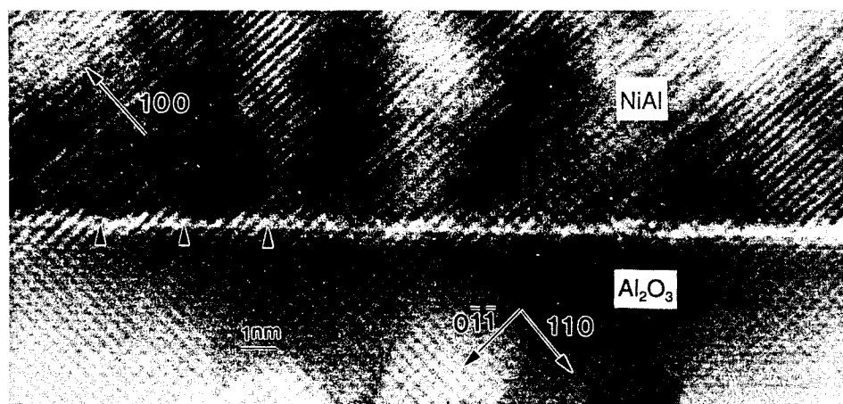
Fig. 8 HREM micrograph of \alpha\text{-Al}_2\text{O}_3/\text{NiAl} interface. Arrows indicate the misfit dislocations in the NiAl
