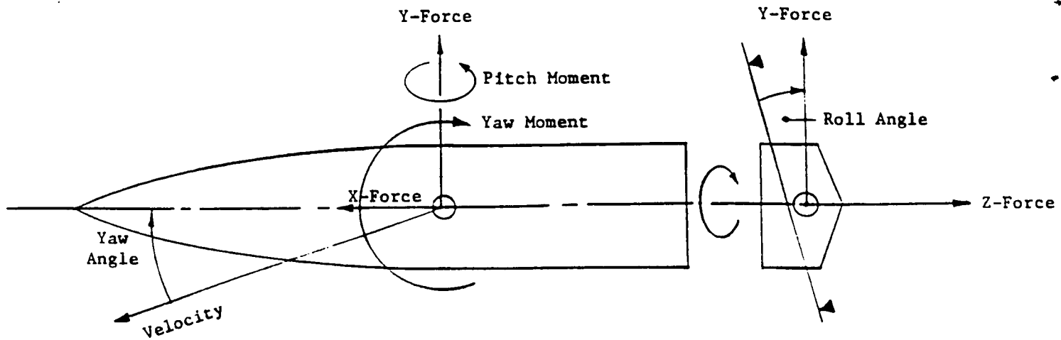
Sketch C3 - Body Axes
