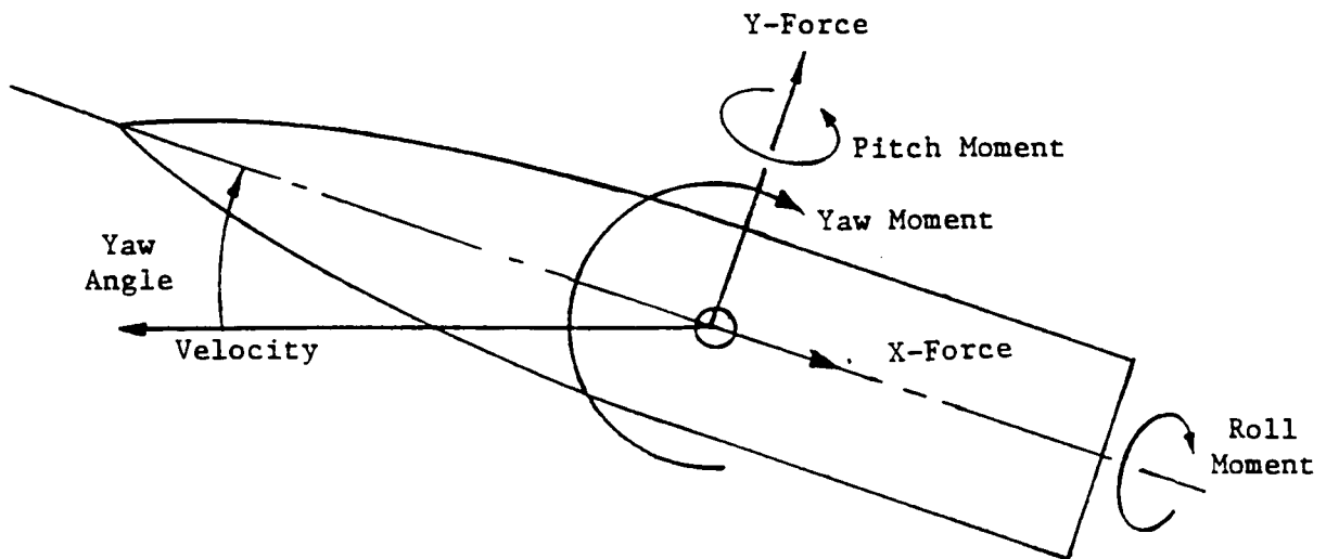
Sketch C1 - Measurement Axes
