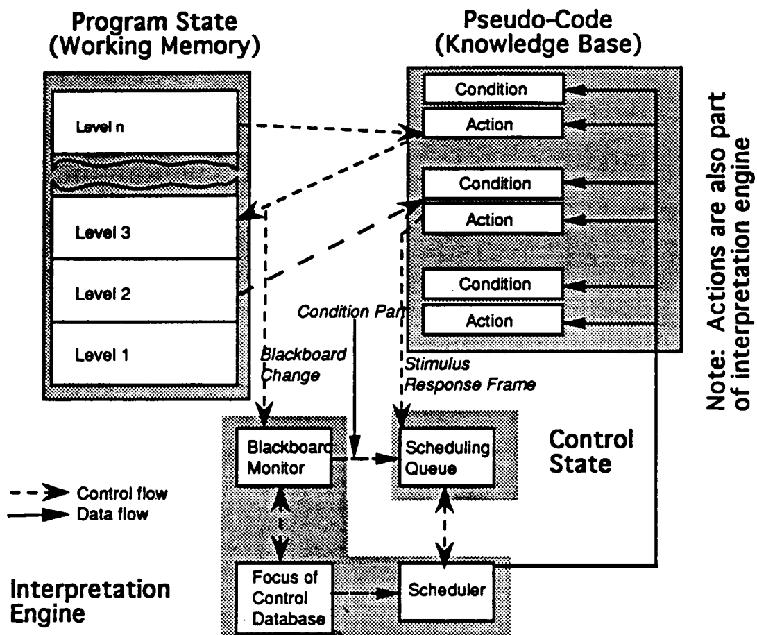
Figure 26: Interpreter View of Hearsay-II
