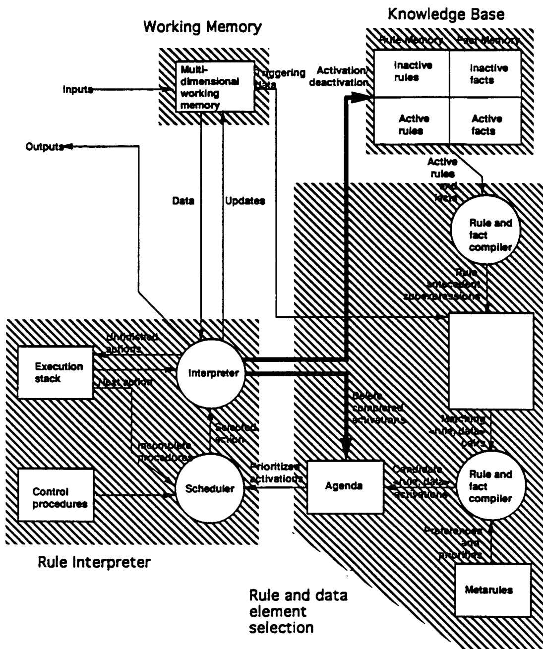
Figure 23: Simplified Rule-Based System
