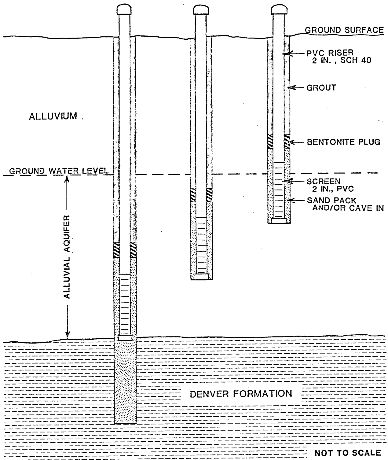
Figure 3. Schematic of cluster wells
