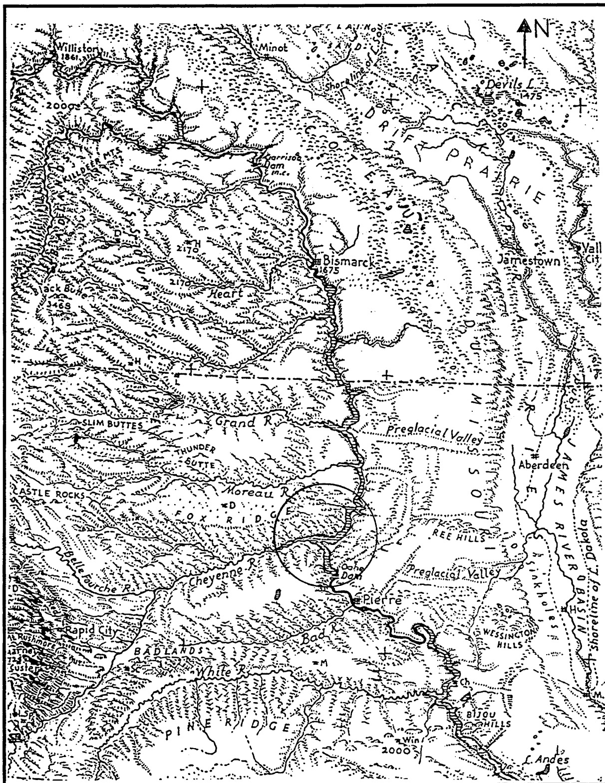
Figure 24. Regional physiographic map showing landforms of South Dakota in relation to the Oahe Reservoir. The map is from Landforms of the United States by Erwin Raisz (6th ed. 1957).
