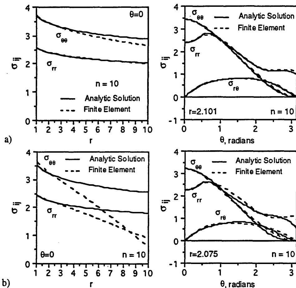
FIG. 3.21— Comparison of a six term analytic solution with finite element predictions for the in-plane stresses of the SENB specimen with an a/W=0.9 : a) J/b\sigma_0=0.003881 , b) J/b\sigma_0=0.032058 .
