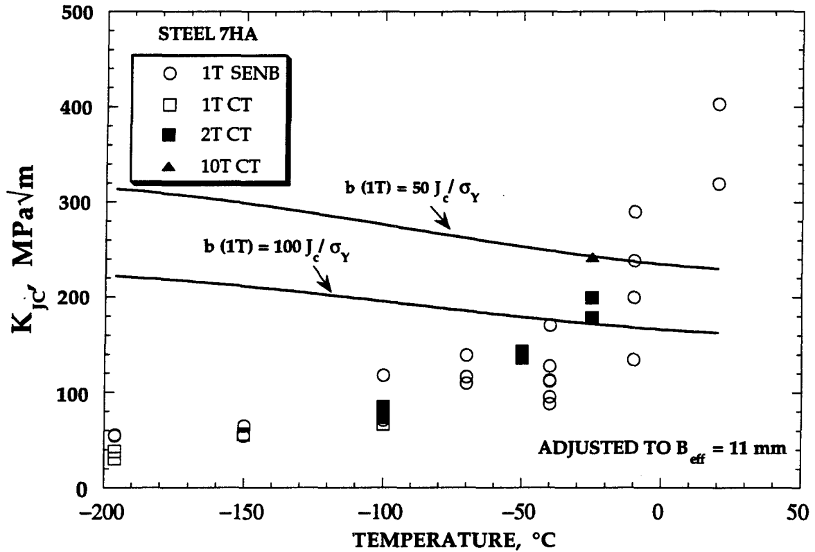
FIGURE 12. Fracture toughness data for Steel 7HA [16].
