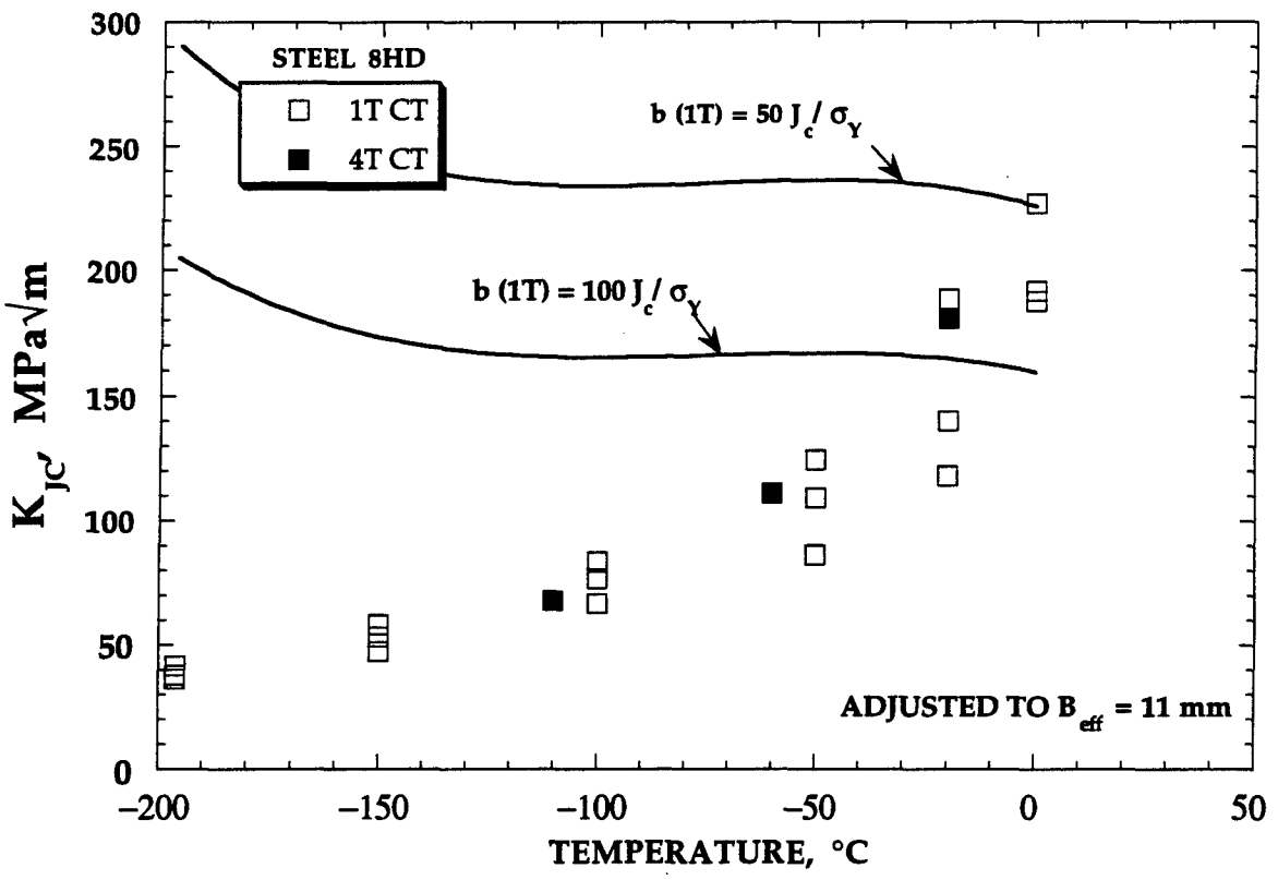
FIGURE 18. Fracture toughness data for Steel 8HD [16].
