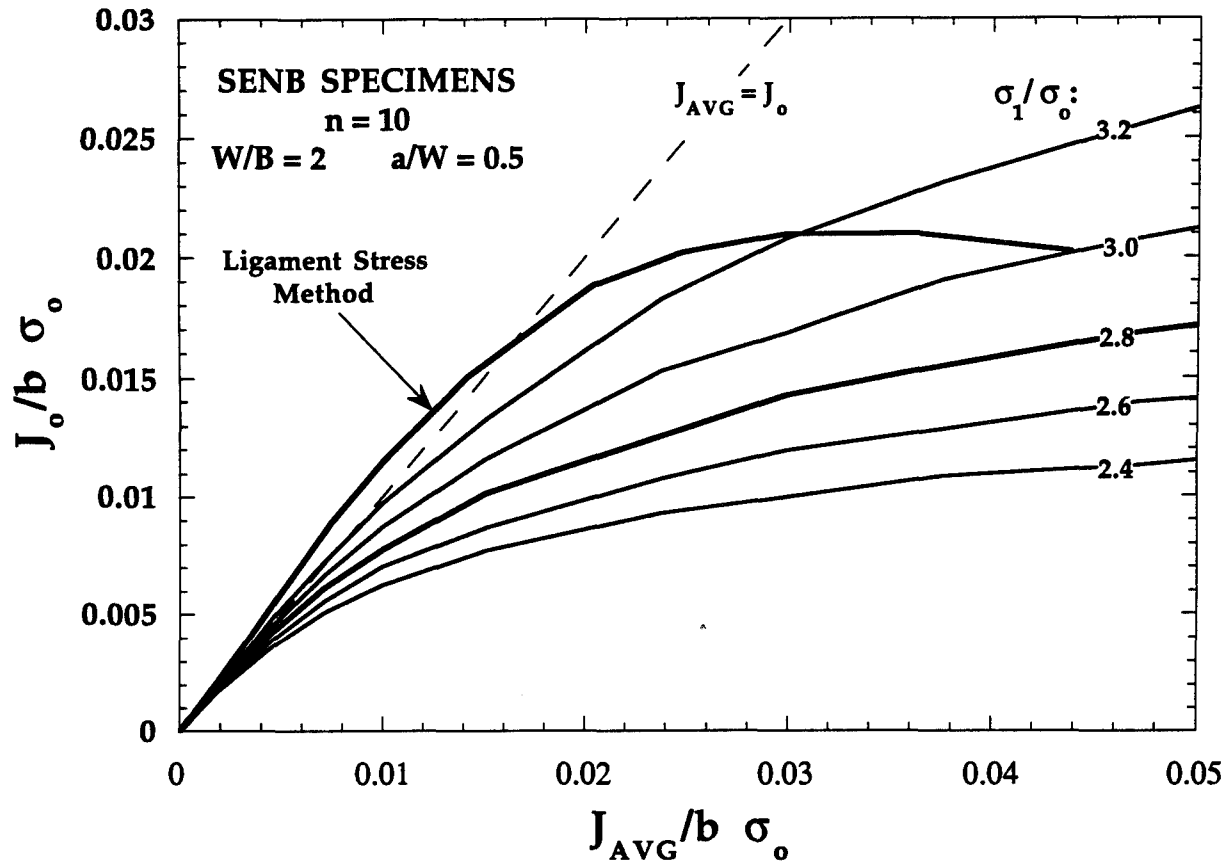
FIGURE 5. Effect of principal stress contour on J_0 estimates for standard B \times 2B SENB specimens.
