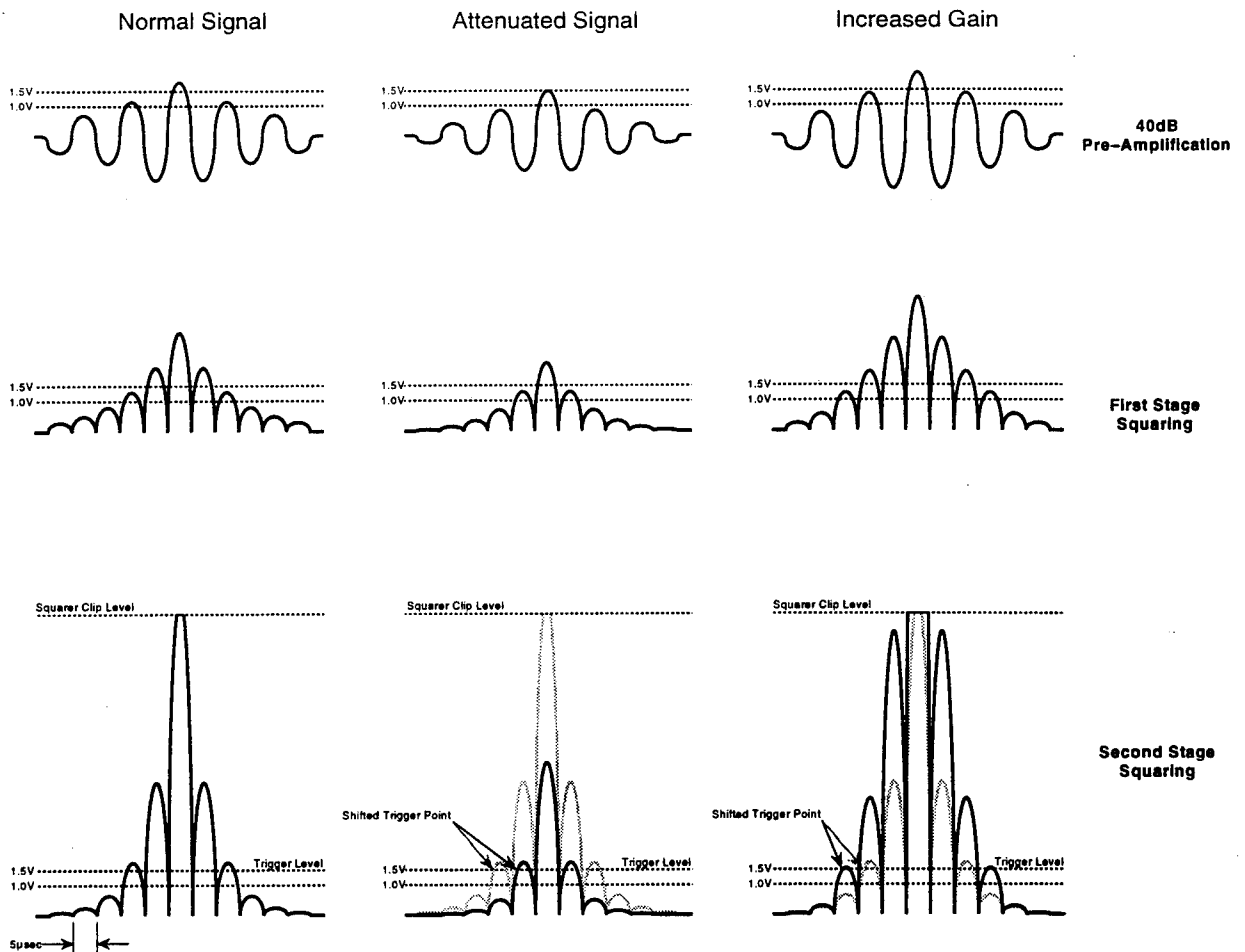
FIGURE 2. Time Shift Concepts
