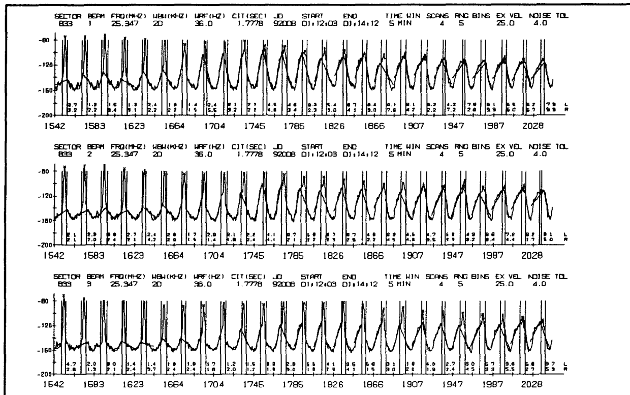
Figure 18 Extremely Strong Ionospheric Clutter
