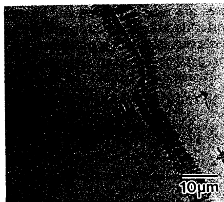
Figure 1. Optical micrographs showing the aging response of (a) TIMETAL 15-3 and (b) TIMETAL 21S after aging for 1 hour at 538°C.
