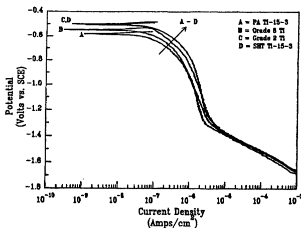
Fig. 12. Cathodic polarization scans for SHT and PA Ti-15-3, grade 2 Ti, and grade 6 Ti exposed to 0.6M NaCl.
