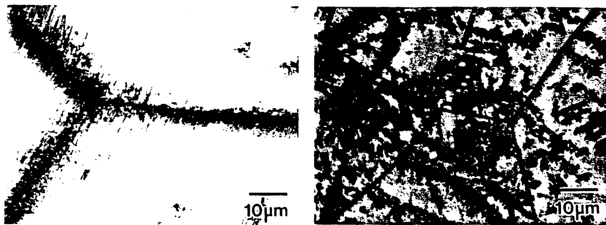
Figure 6: Optical micrographs of underaged (a) Beta 21S and (b) Ti-15-3.
