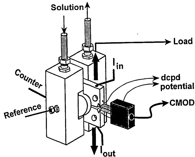
Figure 1. Cell and CT specimen for rising CMOD EAC experiments. ("dcpd" indicates the measurement probes for electrical potential difference due to a direct current, I, through the uncracked portion of the specimen.)
