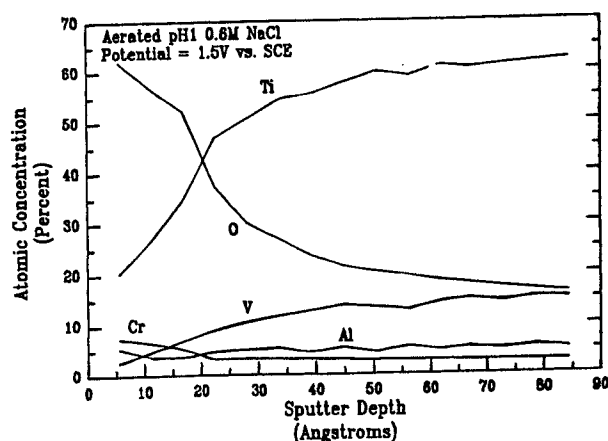
Fig. 10. AES sputter depth profile of SHT Ti-15-3 exposed to aerated 0.6 \text{ M NaCl pH } 1 .
