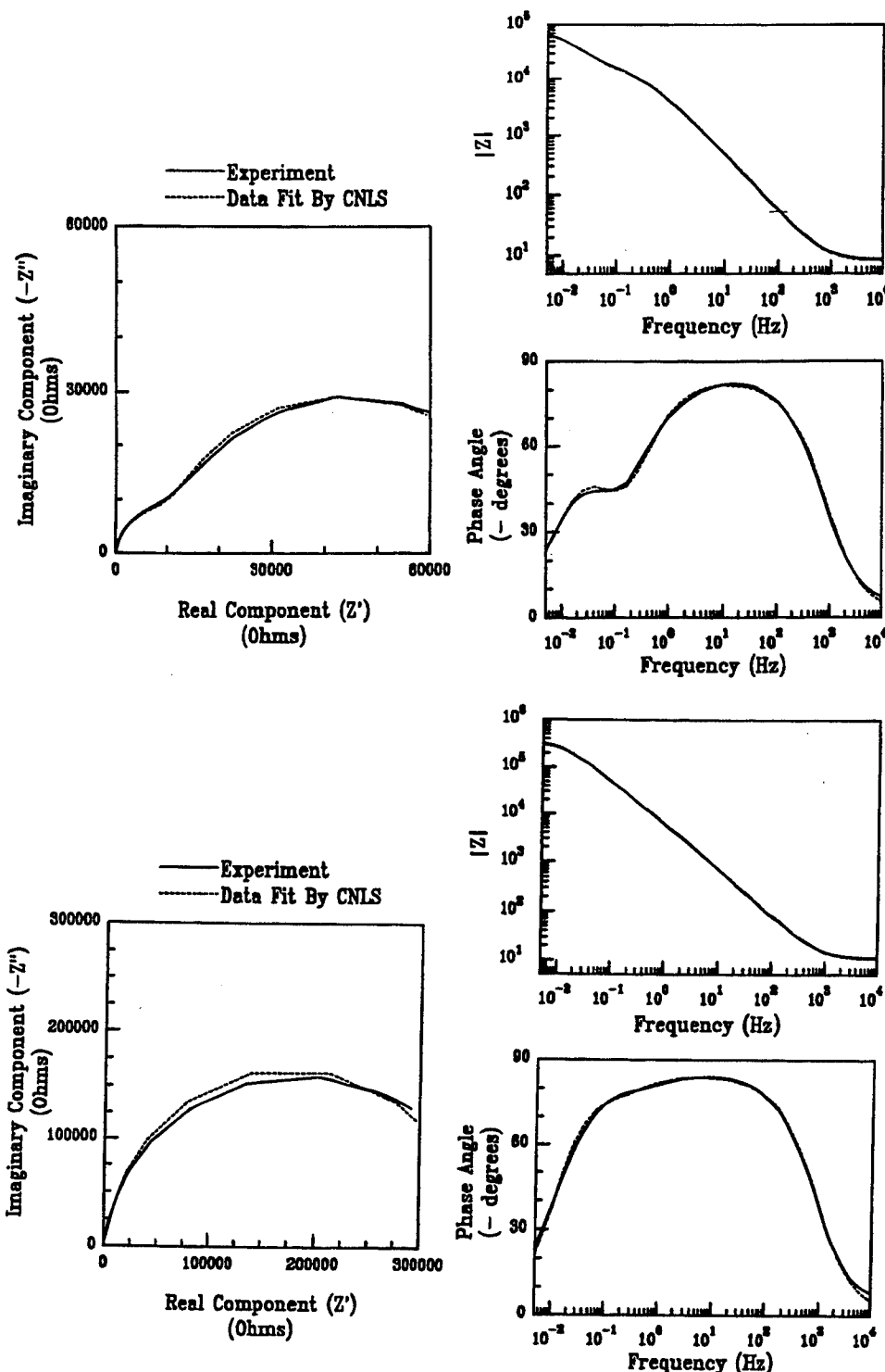
Fig. 5 (a, top) Comparison of experimental data (SHT Ti-15-3, 0.6M NaCl pH 1, E = 1.2 \text{ V}_{\text{SCE}} ) to that obtained by data fitting with CNLS fitting software 19 using the circuit model shown in Fig. 6. (b, bottom) Comparison of experimental data from Fig. 4b (PA Ti-15-3, 0.6M NaCl pH 1, E = 1.2 \text{ V}_{\text{SCE}} ) to that obtained by data fitting with CNLS fitting software 19 using the circuit model shown in Fig. 6.
