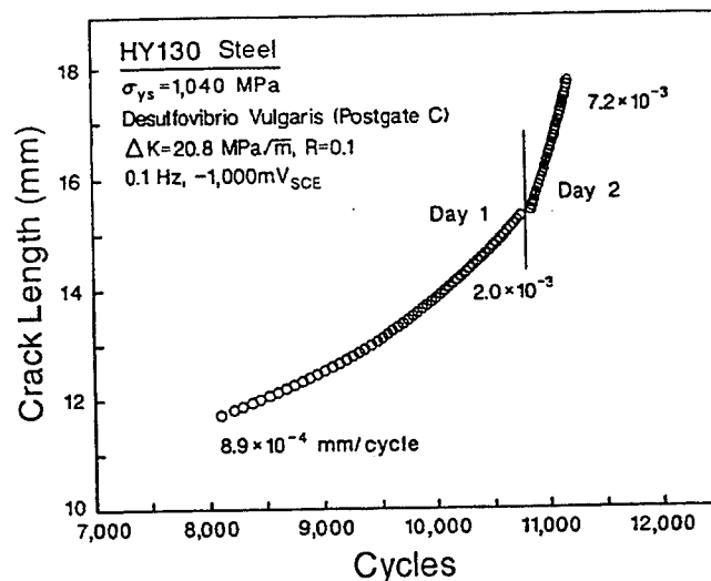
FIGURE 4. Fatigue crack length vs loading cycles for tempered martensitic HY130 steel in Postgate medium C at -1,000 mV SCE , constant \Delta K of 20.8 MPa√m, frequency of 0.1 Hz, and stress ratio of 0.1.
