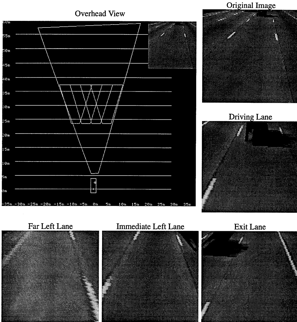
Figure 11. Offramp and lane detection using virtual
