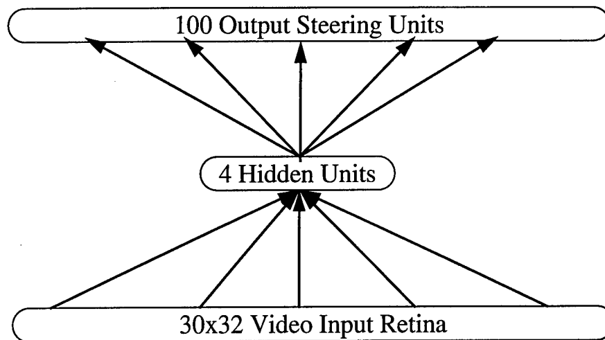
Figure 1. ALVINN network architecture.
