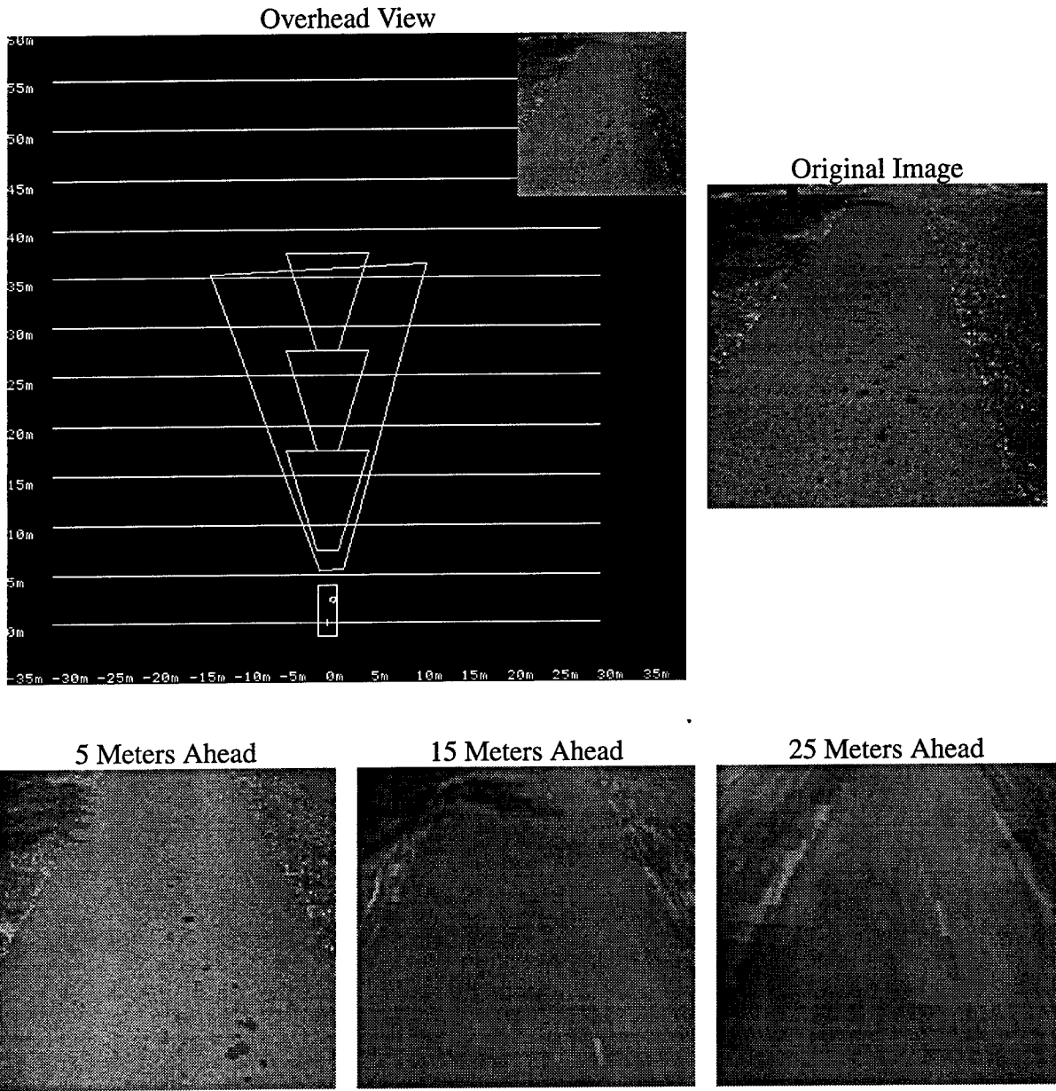
Figure 6. Simulated CBRE images on an unlined, straight, paved path.
