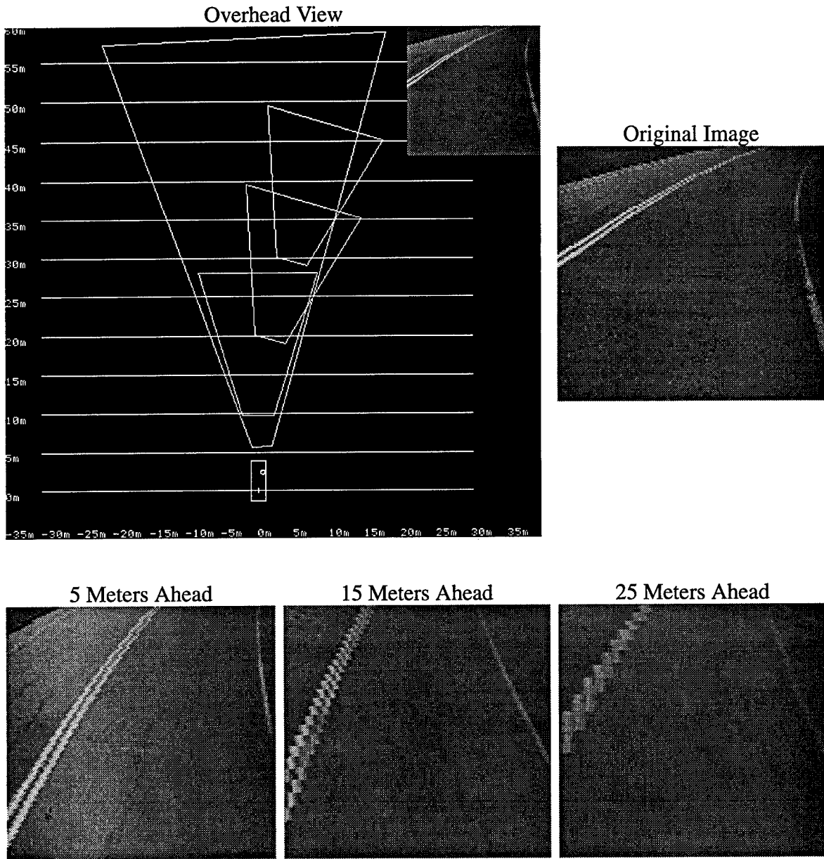
Figure 7. Simulated CBRE images on a lined, curving, city street.
