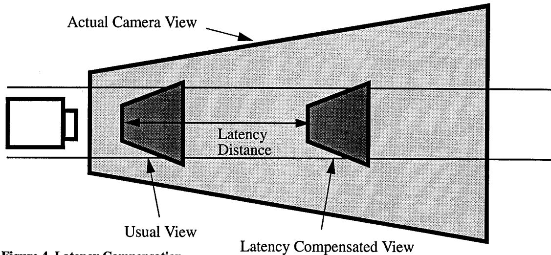
Figure 4. Latency Compensation.
