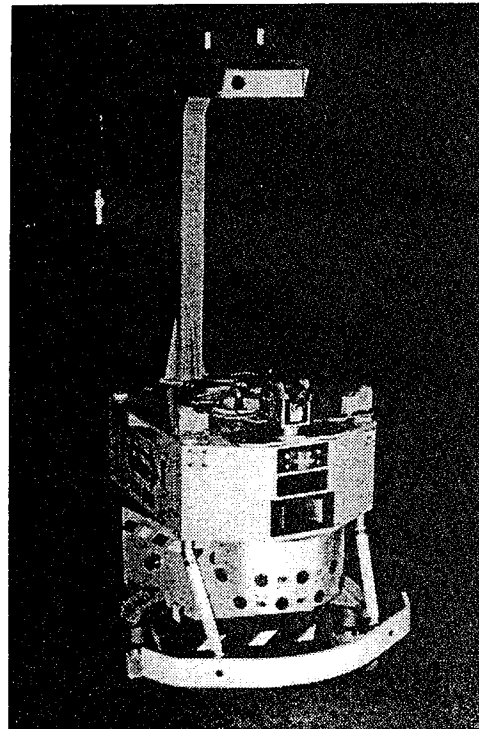
Figure 2. MDARS Interior Platform.
