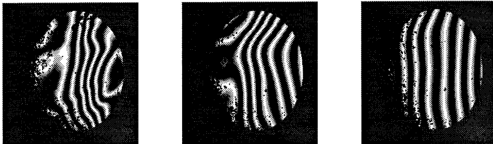
Figure 30. x -direction interferogram patterns for 5.4 cm - 3.6 cm, 3.6 cm - 1.8 cm, and 1.8 cm - 0.0 cm from the shear flow chamber (top view). The fringe separation is proportional to the wavefront slope in the x direction. Gas flow is from right to left. Helium velocity is 8.3 m/sec. Nitrogen velocity is 1.5 m/sec.
