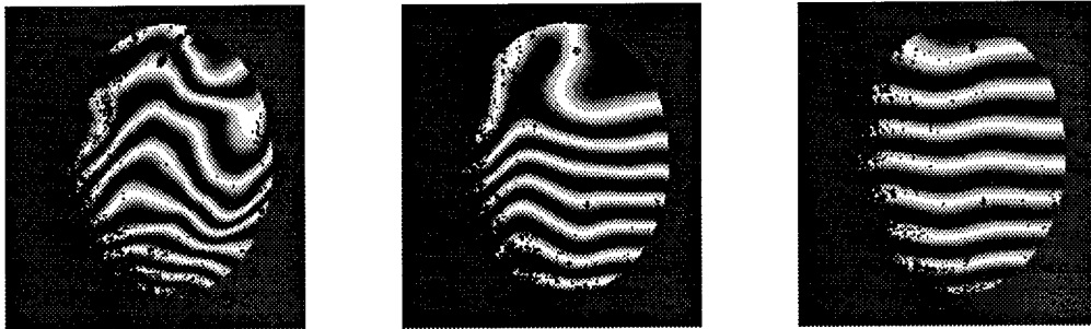
Figure 58. y -direction interferogram patterns for 5.4 cm - 3.6 cm, 3.6 cm - 1.8 cm, and 1.8 cm - 0.0 cm from the shear flow chamber (top view). The fringe separation is proportional to the wavefront slope in the y direction. Gas flow is from right to left. Helium velocity is 8.3 m/sec. Nitrogen velocity is 1.5 m/sec.
