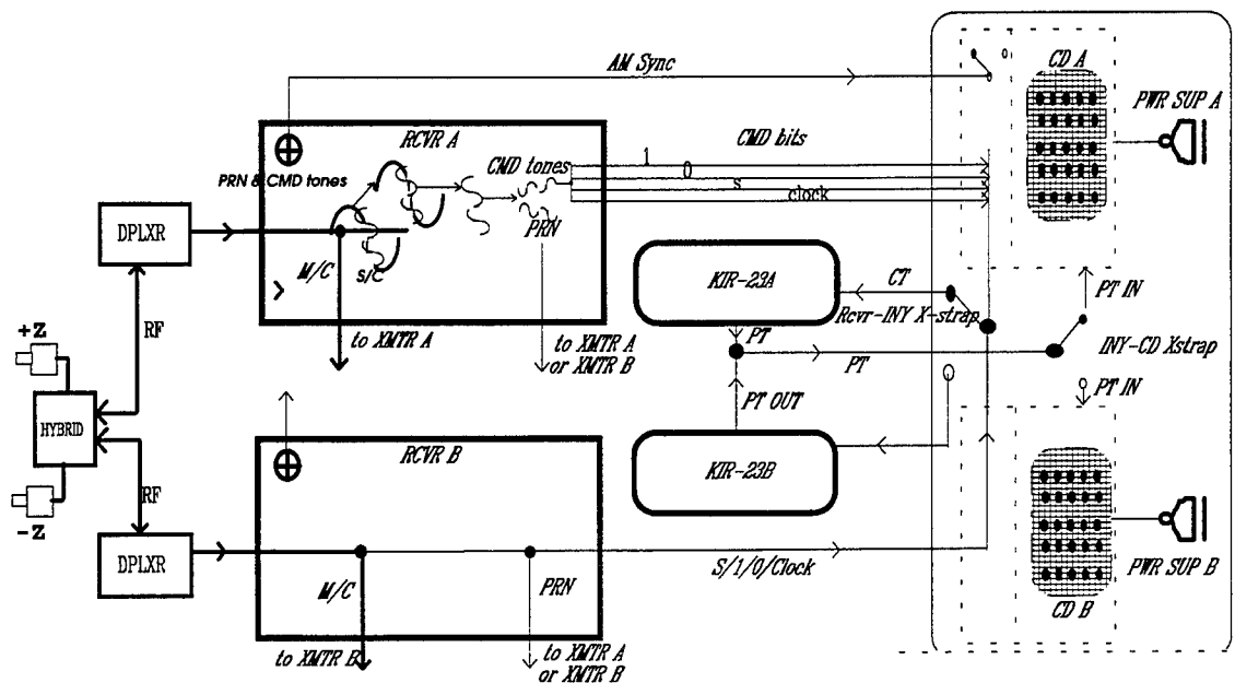
Figure A.2 Uplink Section of the DSCS III TT&C Subsystem (21:9)
