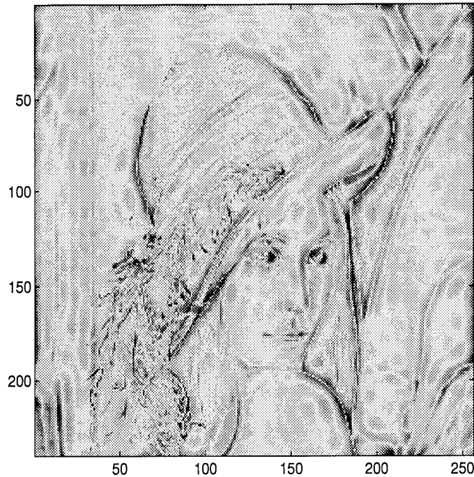
Figure 29. Lenna
