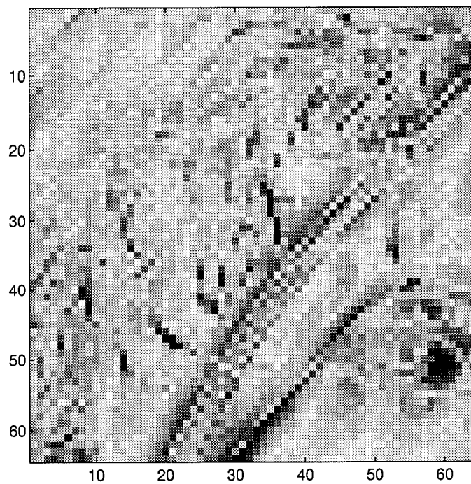
Figure 30. Lenna's Eye
