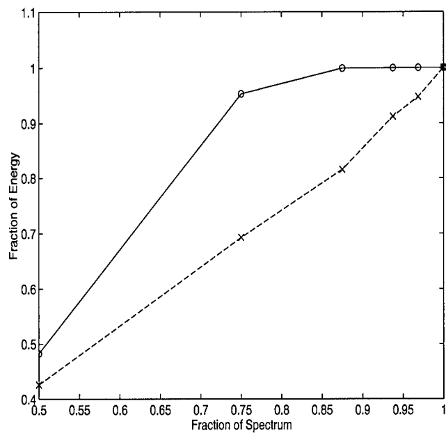
Figure 20. Energy Distribution for a Bandpass Signal. Solid line corresponds to choice of vector length N = 1 at each level. Dotted line corresponds to optimal choice of N = [8, 1, 4, 8, 8] at each level
