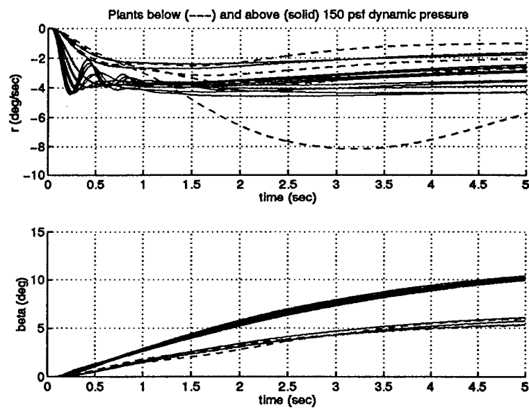
Figure 5.48 Lateral Design \beta_{cmd(max)} Step Responses (2 of 4)
