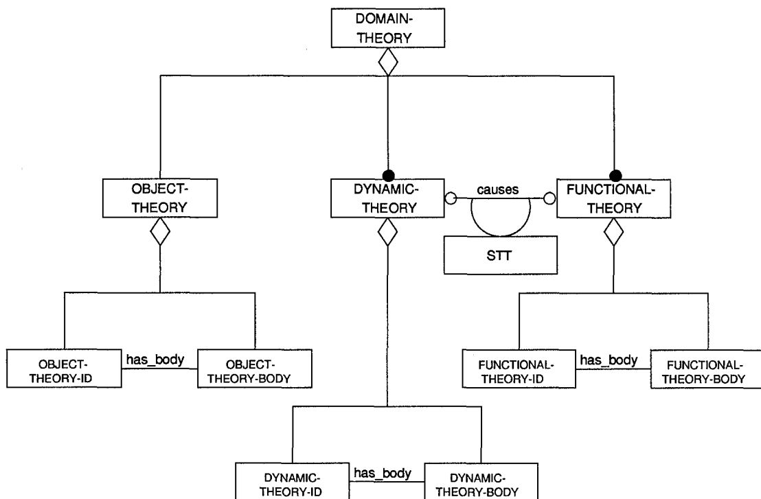
Figure D.1 Unified Domain Theory Model
