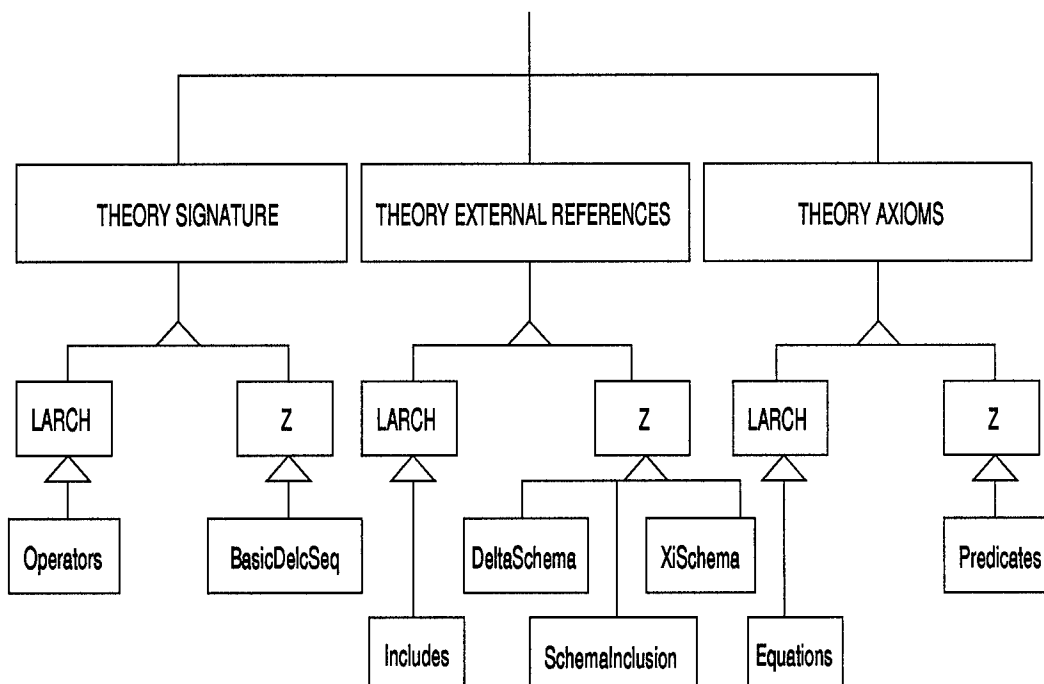
Figure 5.3 Language Inheritance
