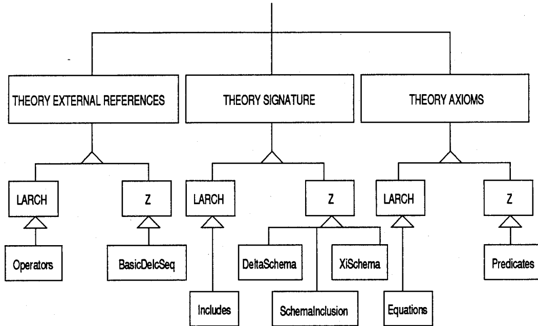
Figure 5.3 Language Inheritance
