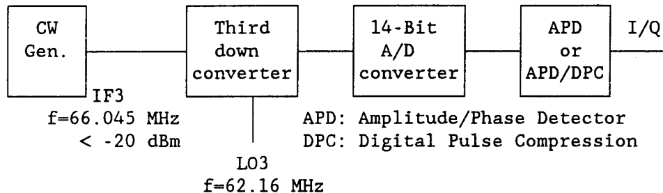
FIGURE 8.4-1. I AND Q PHASE AND AMPLITUDE ERRORS CONFIGURATION
