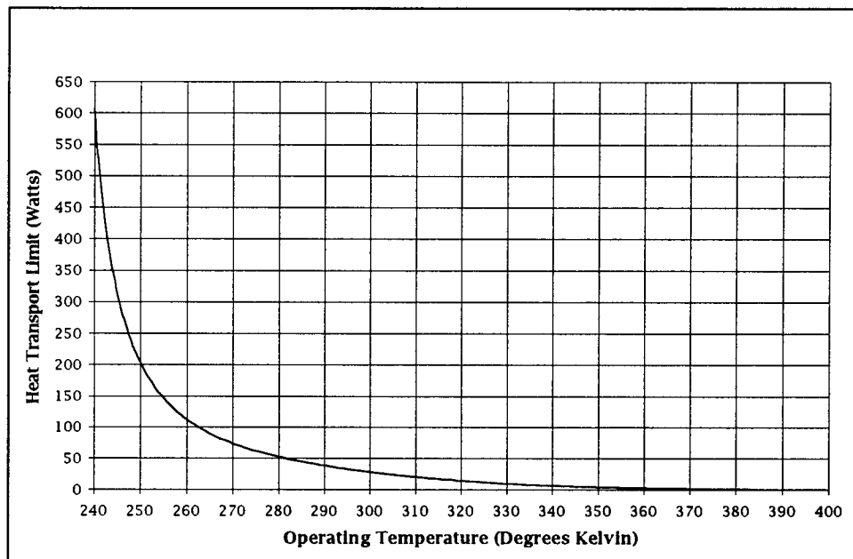
Figure A.4 Boiling Heat Transport Limit
