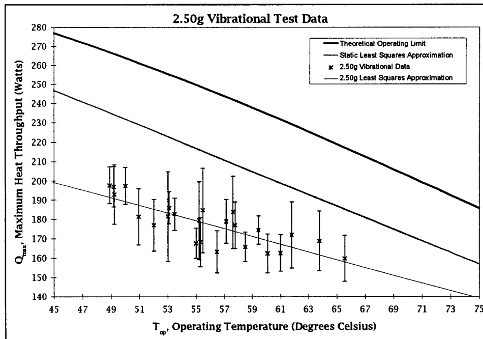
Figure 4.3 Q_{max} versus T_{op} : 2.50g Vibrational Test Case
