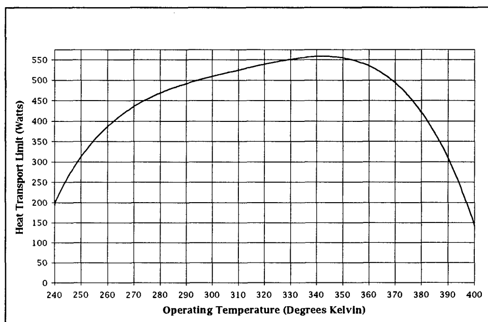
Figure A.2 Entrainment Heat Transport Limit
