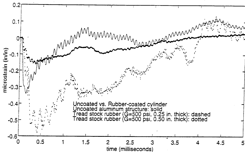
Figure 64. Hoop strain at position B for uncoated vs. coated aluminum cylinders of varying coating thicknesses and constant shear modulus of 500 psi
